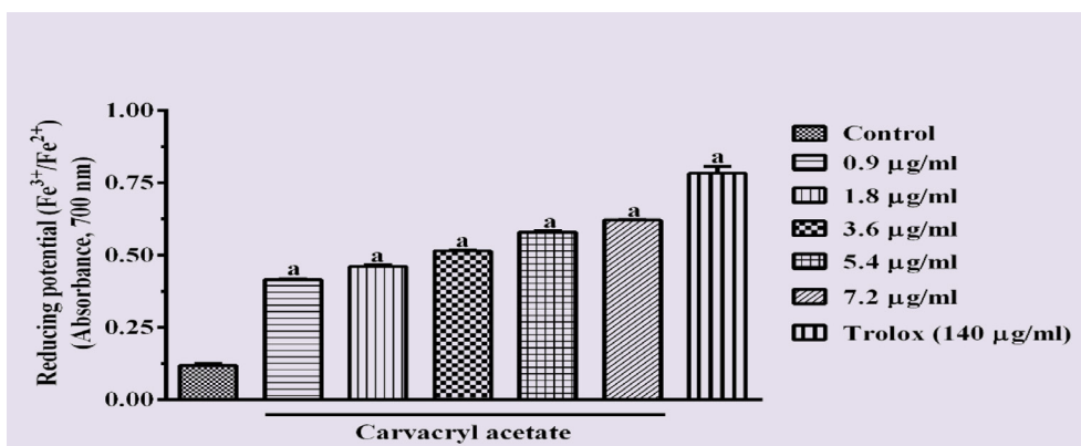
Figure 4. Reduction potential ( \text{Fe}^{3+}/\text{Fe}^{2+} ) of carvacryl acetate. The results represent the mean ± S.E.M. of the values of in vitro inhibition, n=5, of the experiments in duplicate. The Trolox (140 µg/mL) was used as standard antioxidant. * p < 0.05 versus control (without carvacryl acetate) (ANOVA and Newman-Keuls as post hoc test)
