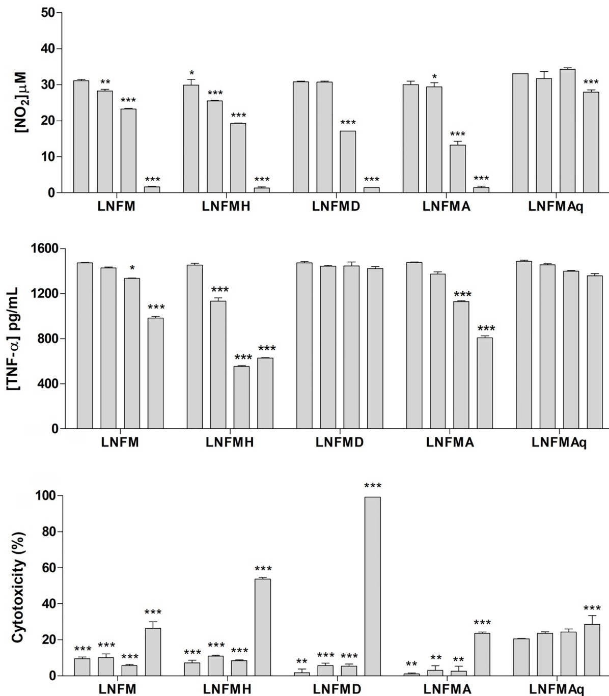
Figure 1. Effect of L. nepetifolia leaves methanolic extract (LNFM) and fractions – hexane (LNFMH), dichloromethane (LNFMD), ethyl acetate (LNFMA), and aqueous LNFMAq) - in NO and TNF- \alpha production on LPS-stimulated RAW 264.7 macrophages and cytotoxic evaluation. Tested concentrations from the left to right were: 0.8, 4, 20, and 100 \mu\text{g/mL} .
