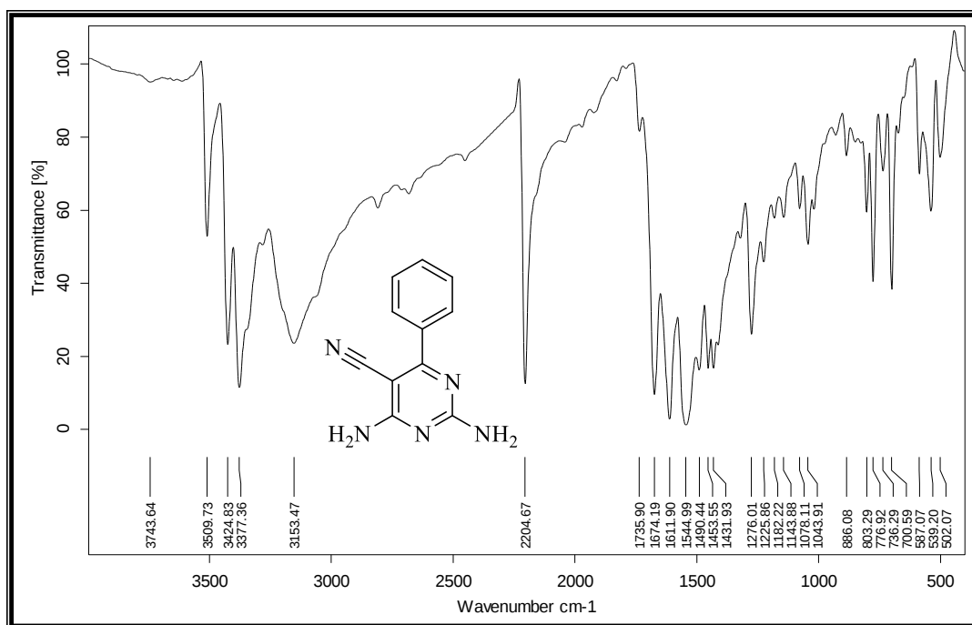
Figure 3S. IR spectrum of 2,4-diamino-6-(phenyl)pyrimidine-5-carbonitrile ( 4b )
