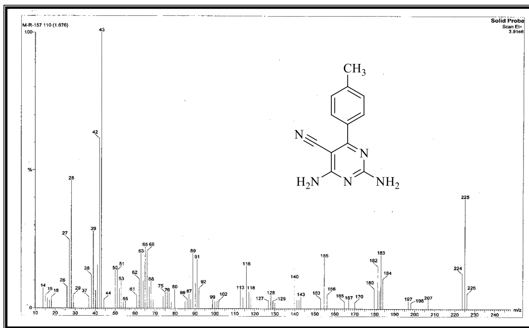
Figure 5S. Mass spectrum of 2,4-diamino-6-p-tolylpyrimidine-5-carbonitrile ( 4c )
