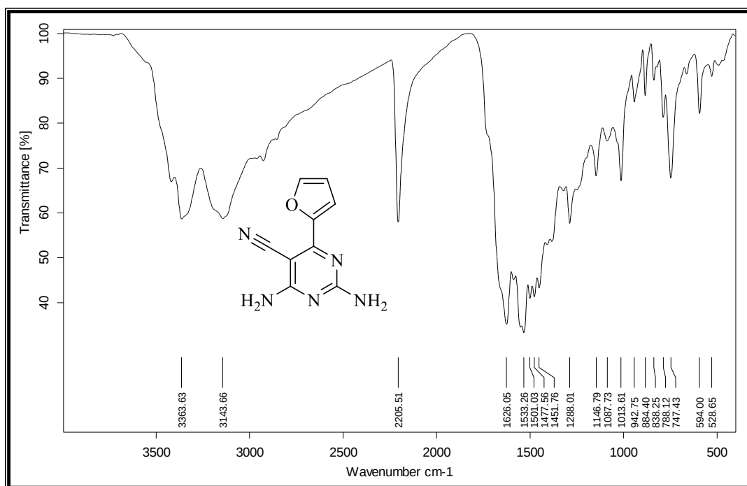
Figure 17S. IR spectrum of 2,4-diamino-6-(furan-2-yl)pyrimidine-5-carbonitrile ( 4h )
