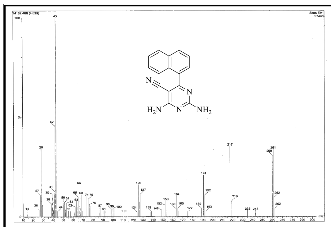
Figure 16S. Mass spectrum of 2,4-diamino-6-(naphthalen-1-yl)pyrimidine-5-carbonitrile ( 4g )
