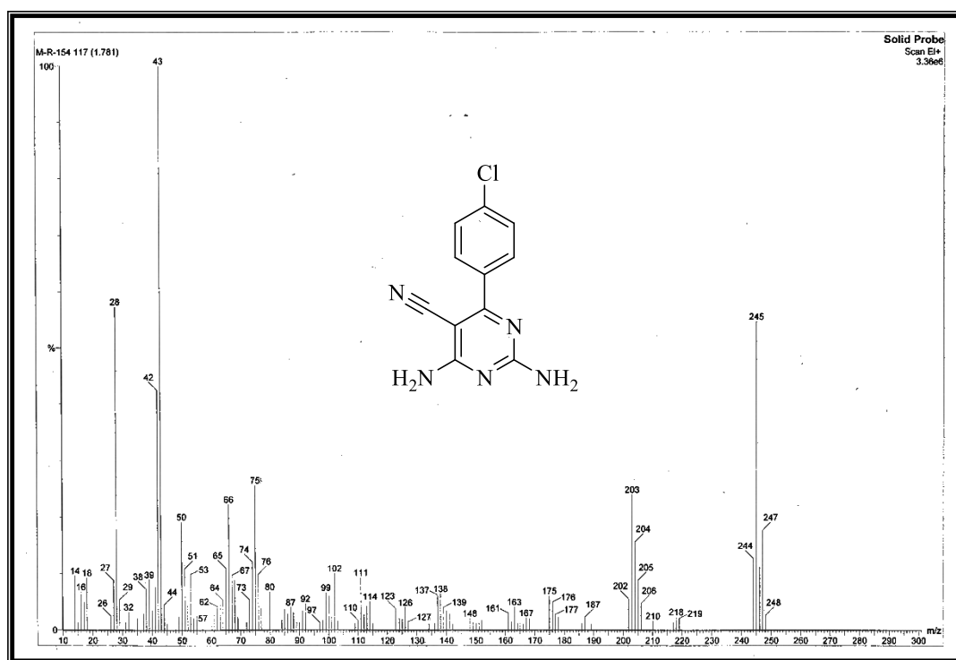
Figure 2S. Mass spectrum of 2,4-diamino-6-(4-chlorophenyl)pyrimidine-5-carbonitrile (4a)
