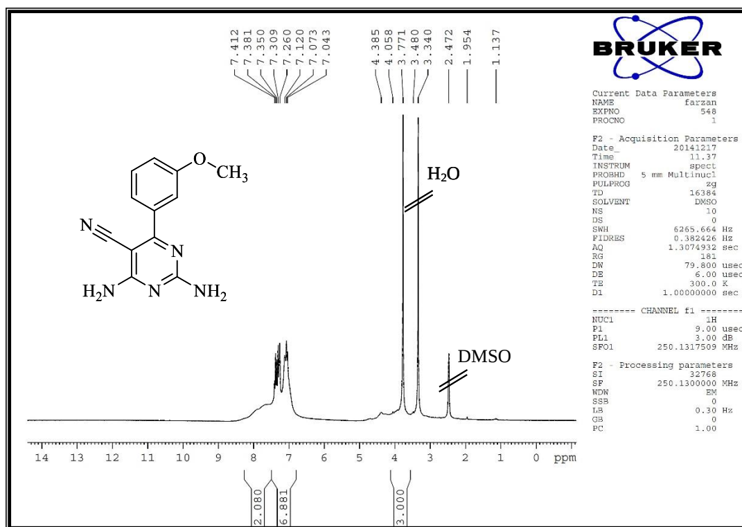
Figure 9S. 1 H NMR of 2,4-diamino-6-(3-methoxyphenyl)pyrimidine-5-carbonitrile ( 4e )
