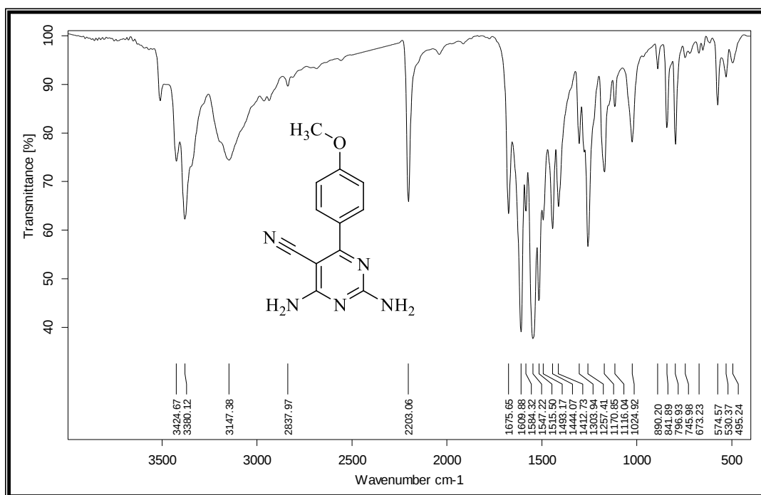
Figure 6S. IR spectrum of 2,4-diamino-6-(4-methoxyphenyl)pyrimidine-5-carbonitrile ( 4d )
