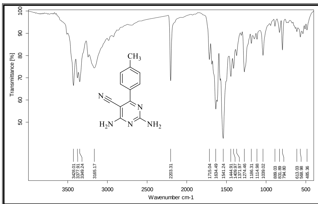
Figure 4S. IR spectrum of 2,4-diamino-6-p-tolylpyrimidine-5-carbonitrile ( 4c )
