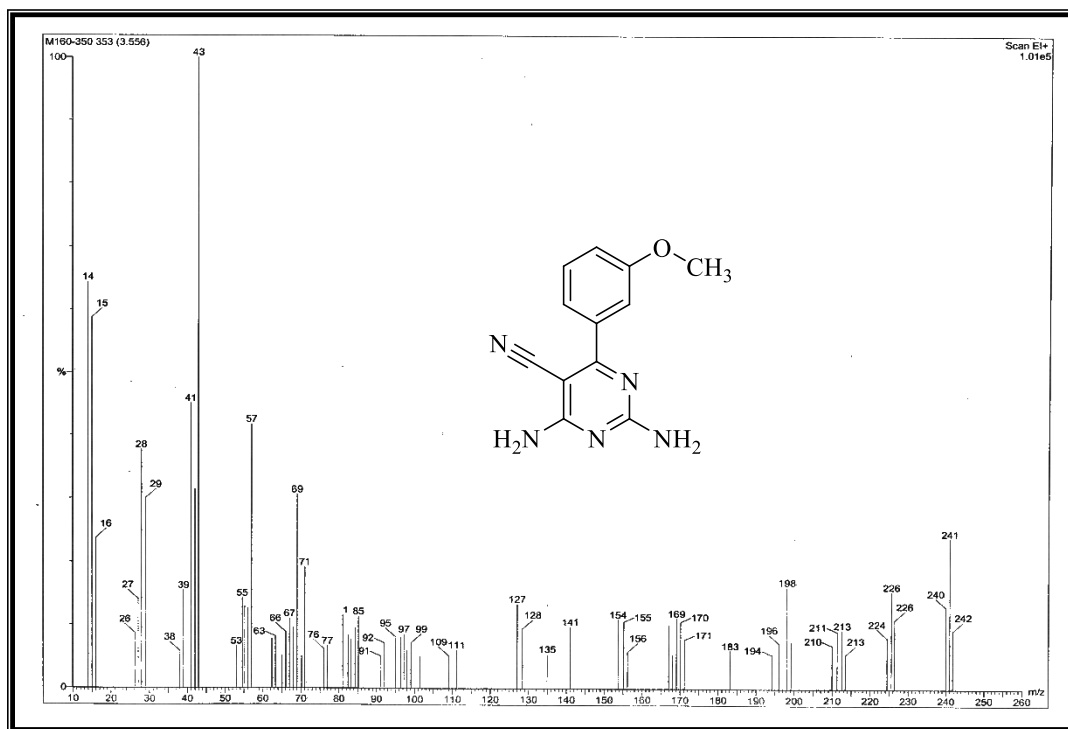
Figure 11S. Mass spectrum of 2,4-diamino-6-(3-methoxyphenyl)pyrimidine-5-carbonitrile (4e)
