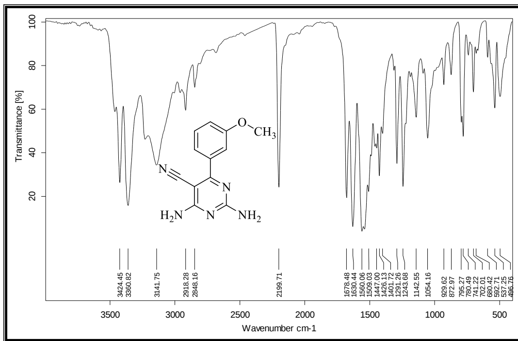
Figure 8S. IR spectrum of 2,4-diamino-6-(3-methoxyphenyl)pyrimidine-5-carbonitrile ( 4e )
