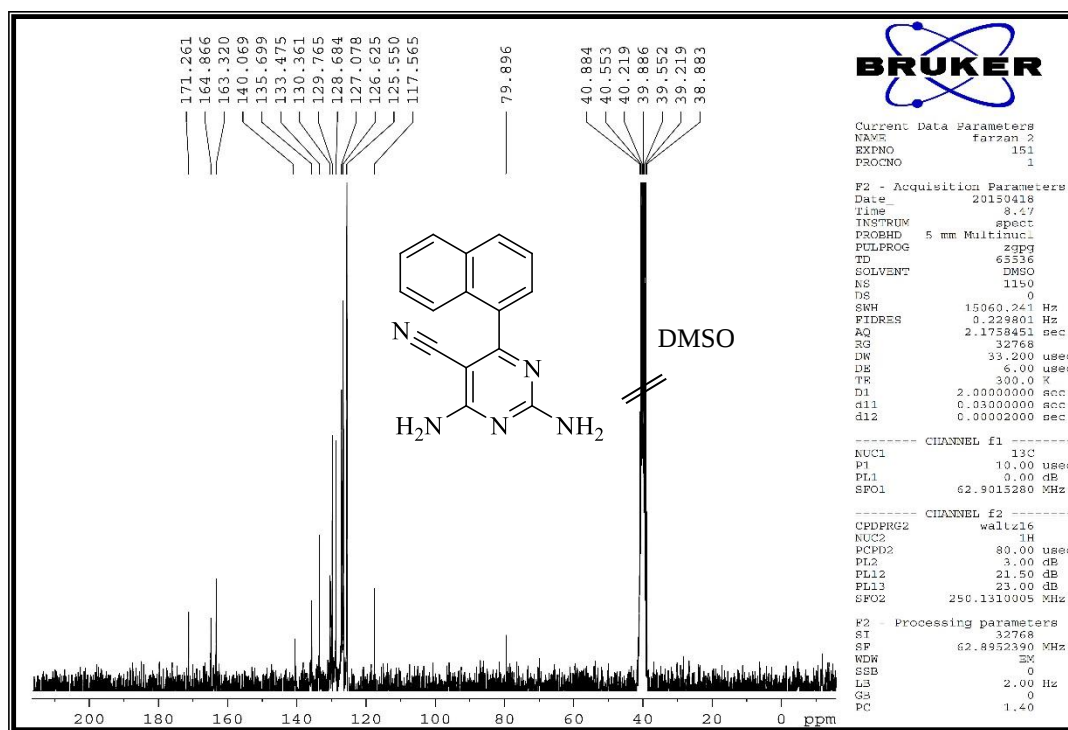
Figure 15S. ^{13}\text{C} NMR of 2,4-diamino-6-(naphthalen-1-yl)pyrimidine-5-carbonitrile ( 4g )
