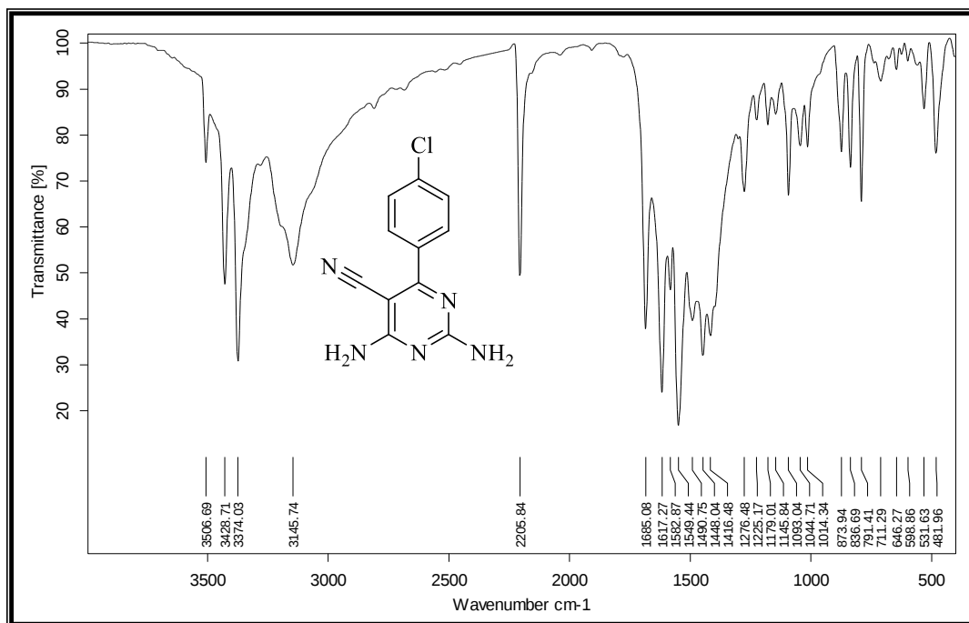
Figure 1S. IR spectrum of 2,4-diamino-6-(4-chlorophenyl)pyrimidine-5-carbonitrile (4a)
