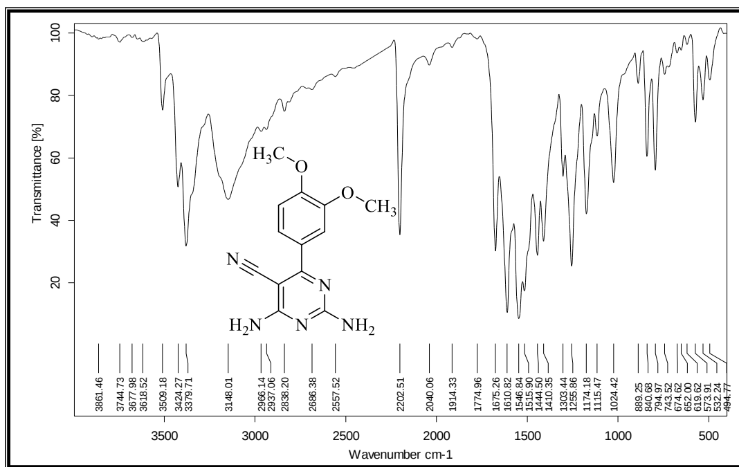
Figure 18S. IR spectrum of 2,4-diamino-6-(3,4-dimethoxyphenyl)pyrimidine-5-carbonitrile ( 4i )
