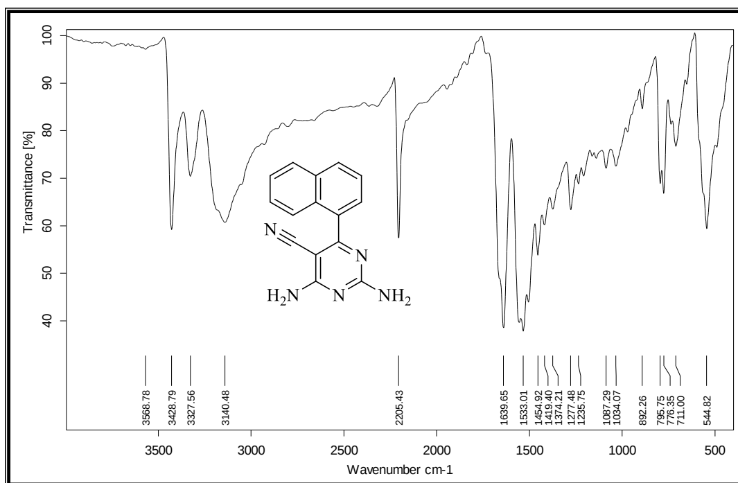
Figure 13S. IR spectrum of 2,4-diamino-6-(naphthalen-1-yl)pyrimidine-5-carbonitrile (4g)
