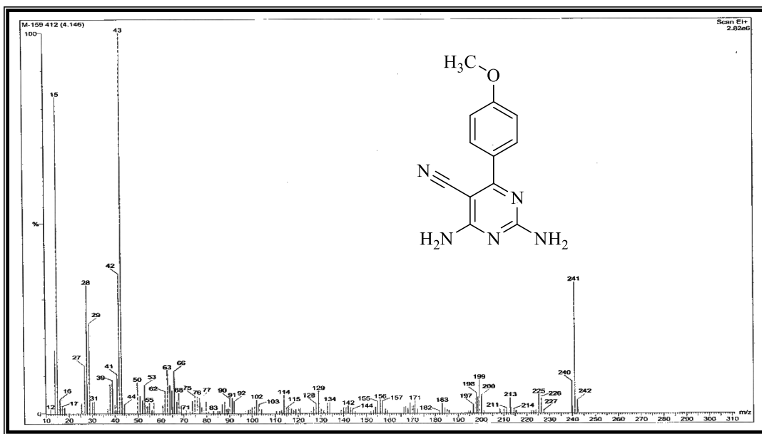
Figure 7S. Mass spectrum of 2,4-diamino-6-(4-methoxyphenyl)pyrimidine-5-carbonitrile ( 4d )
