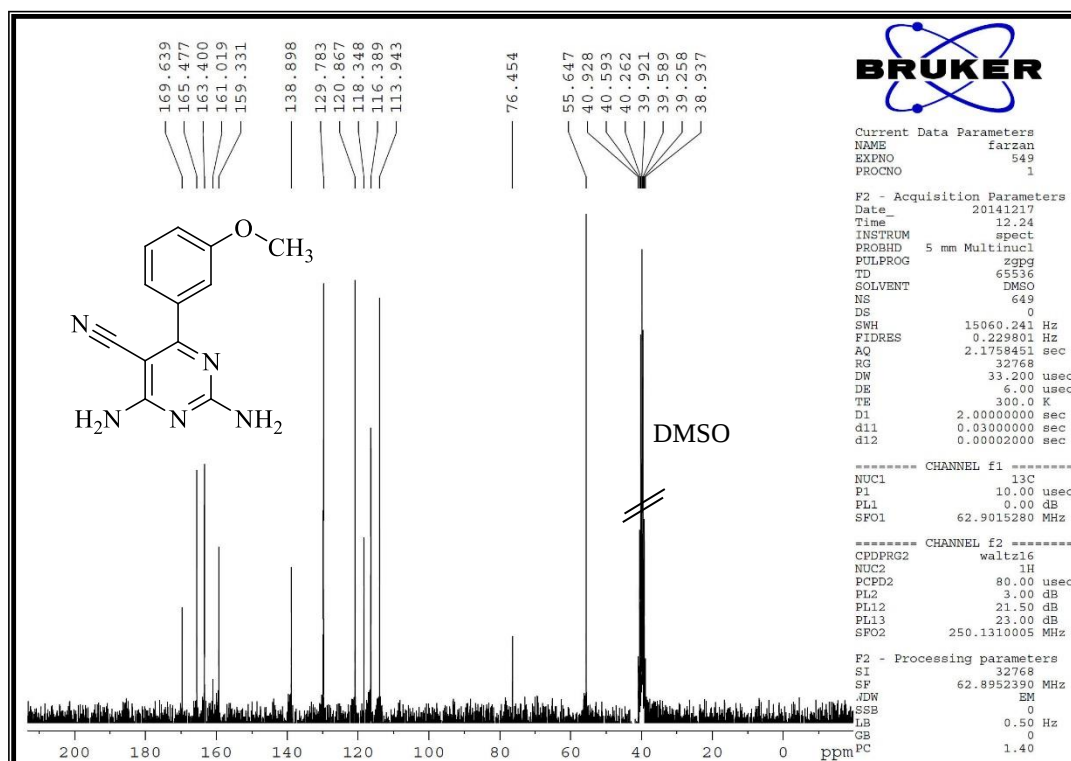
Figure 10S. 13 C NMR of 2,4-diamino-6-(3-methoxyphenyl)pyrimidine-5-carbonitrile ( 4e )
