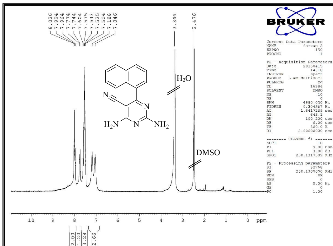
Figure 14S. 1 H NMR of 2,4-diamino-6-(naphthalen-1-yl)pyrimidine-5-carbonitrile (4g)
