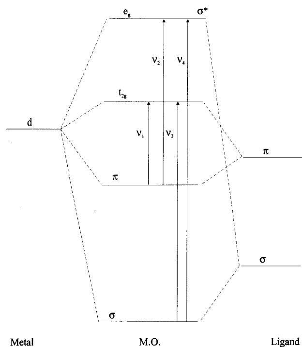
Figure 2. A simplified molecular orbital diagram illustrating the potential ligand-to-metal charge transfer transitions. Transitions to t_{2g} are absent in the low spin Fe(II) complexes.
