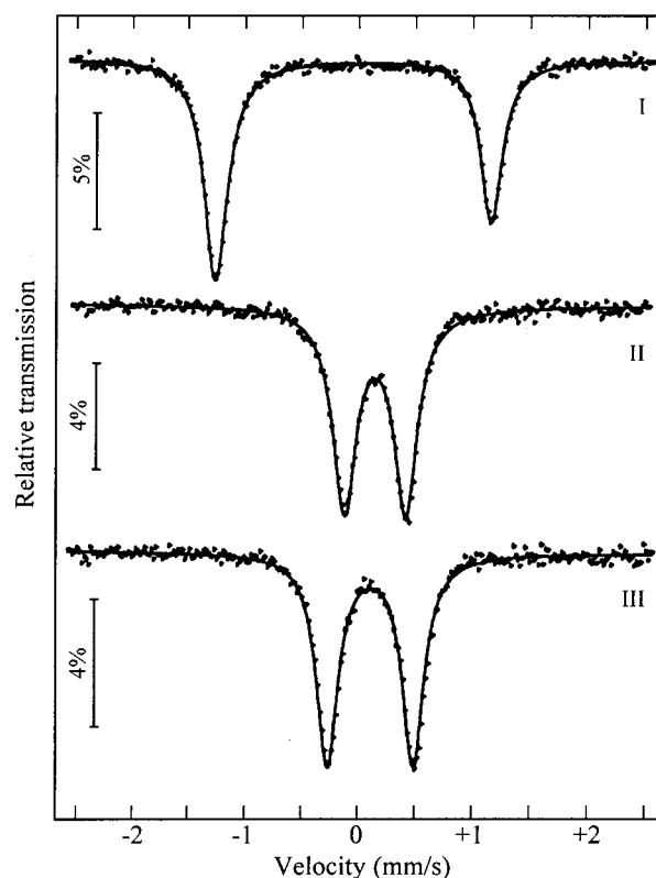
Figure 3. Mössbauer spectra at 298 K of the complexes: [Fe(HAPT)Cl 2 ] (I), [Fe(HAPT) 2 ]Cl 2 (II) and [Fe(APT) 2 ] (III).
