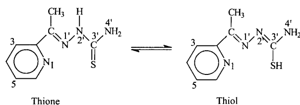
Figure 1. Structure of the ligand 2-acetylpyridine thiosemicarbazone under the thione and thiol tautomeric forms.
