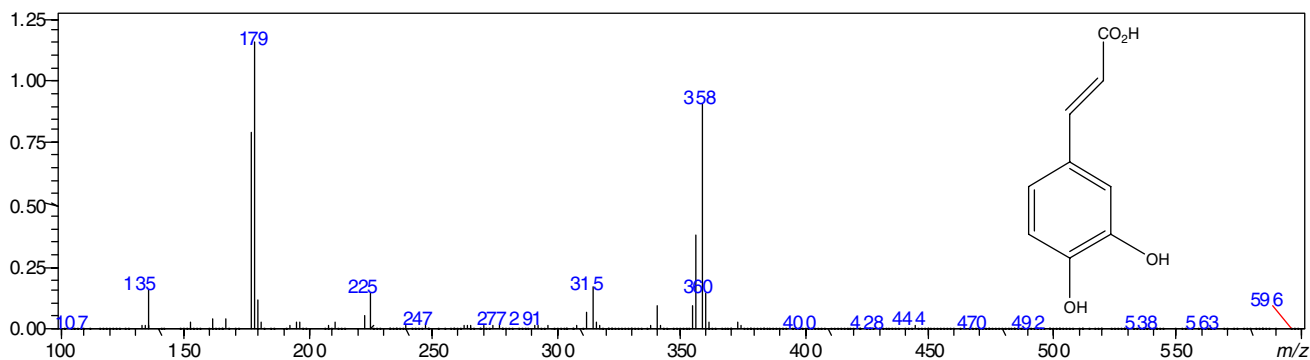
Figure S2. Negative ESI-MS of caffeic acid.
