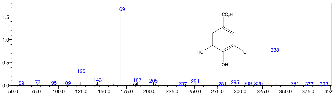
Figure S1. Negative ESI-MS of gallic acid.
