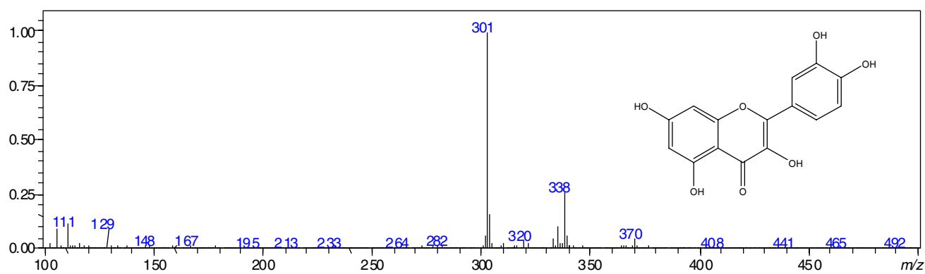
Figure S4. Negative ESI-MS of quercetin.
