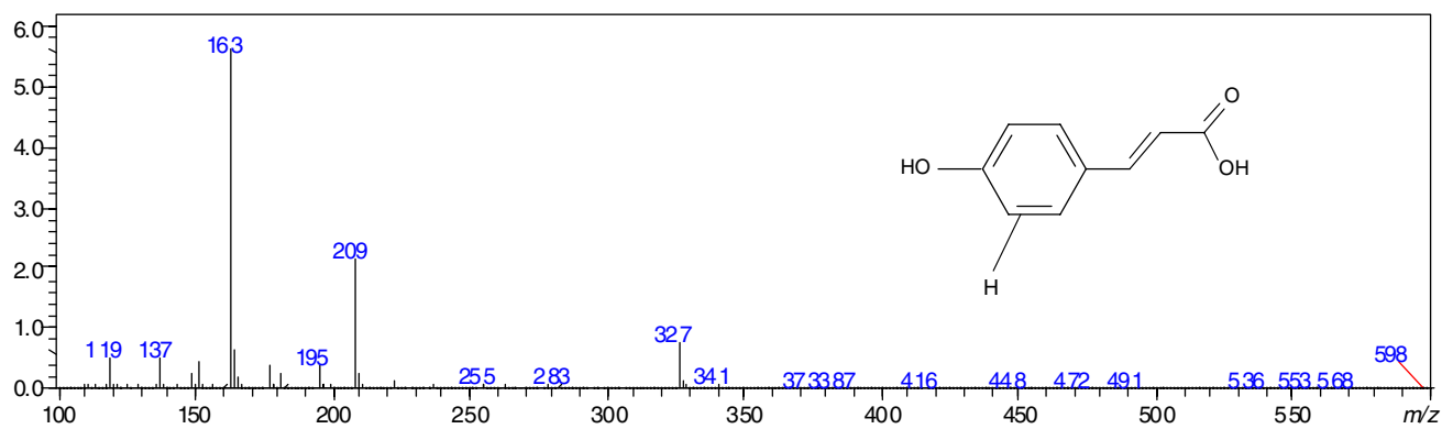
Figure S3. Negative ESI-MS of p -coumaric acid.
