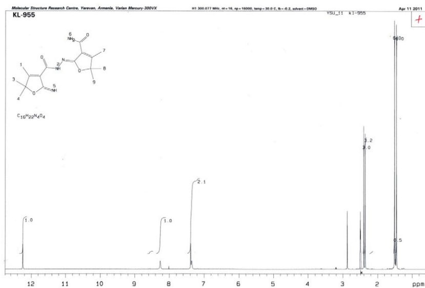
Figure S2. 1 H NMR spectrum (300 MHz, DMSO- d 6 ) of compound 5a.
