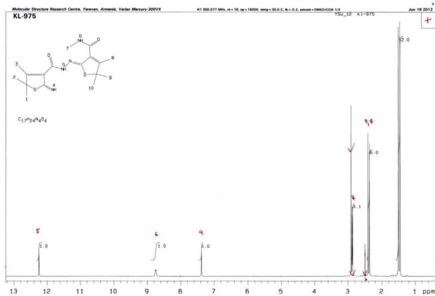
Figure S5. ^1H NMR spectrum (300 MHz, DMSO- d_6 :CCl _4 , 1:3) of compound 5e .
