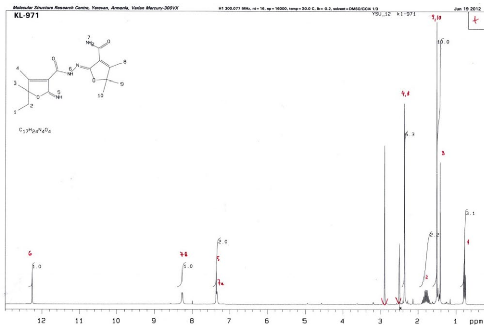
Figure S3. 1 H NMR spectrum (300 MHz, DMSO- d 6 :CCl 4 , 1:3) of compound 5b .
