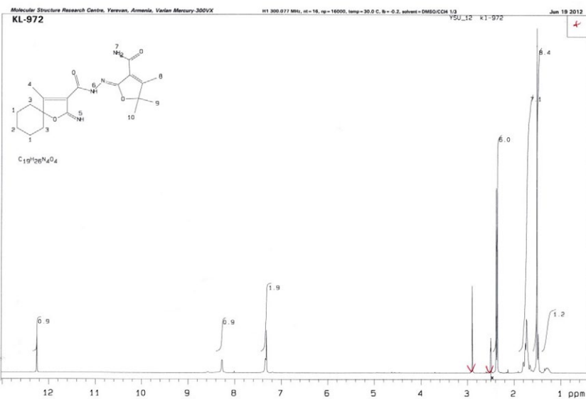
Figure S4. 1 H NMR spectrum (300 MHz, DMSO- d 6 :CCl 4 , 1:3) of compound 5d .
