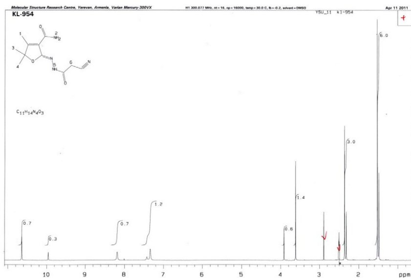
Figure S1. 1 H NMR spectrum (300 MHz, DMSO- d 6 ) of compound 3a.
