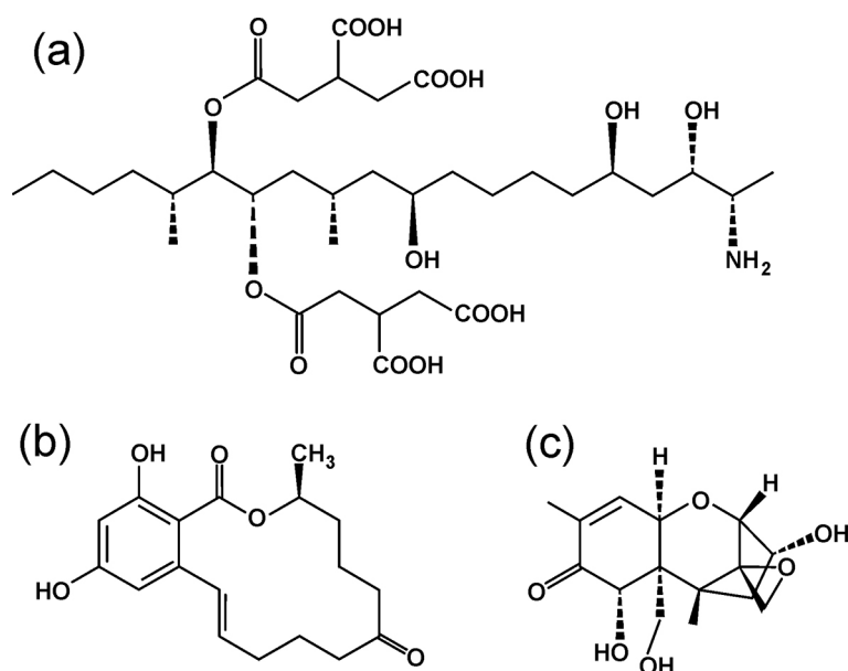
Figure S1. Schematic representation of the chemical structure of fumonisin B 1 (a), zearalenone (b) and deoxynivalenol (c).
