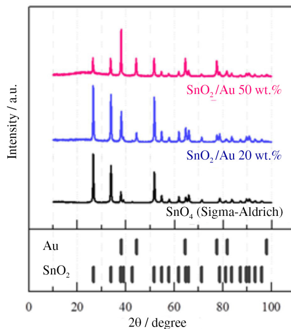
Figure S2. XRD pattern for the studied electrocatalysts: Au (PDF No. 00-004-0784), and SnO 2 (PDF No. 00-021-1250).
