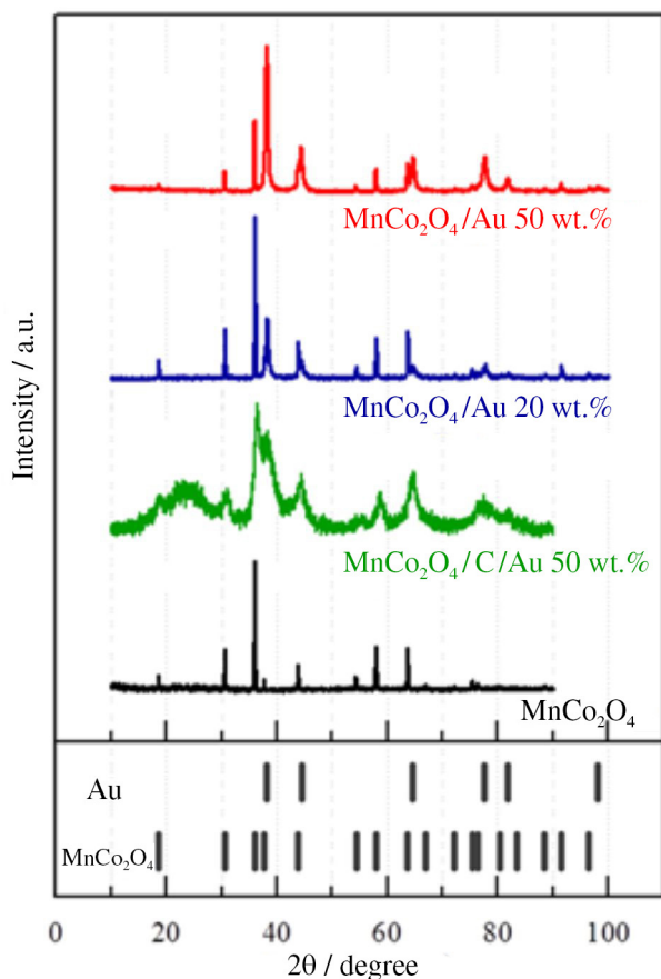
Figure S1. XRD pattern for the studied electrocatalysts: Au (PDF No. 00-004-0784), and MnCo 2 O 4 (PDF No. 00-023-1237).
