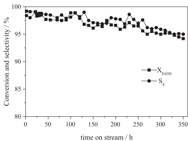
Figure S1. The lifetime of AT0.4 catalyst.
