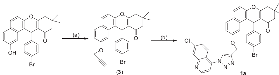
Scheme 4. Sequential synthesis of 1a . Reagents and conditions: (a) PEG-400, K_2CO_3 (1 eq.), 80^\circ C ; (b) PEG-400, 4-azido-7-chloroquinoline (1.0 eq.), CuSO_4 \cdot 5H_2O (10 mol%), sodium ascorbate (15 mol%), 80^\circ C .
