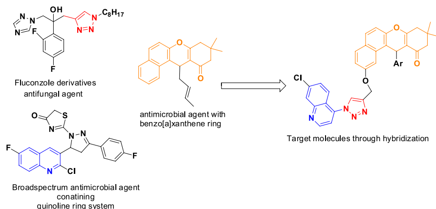
Scheme 1. Structure of bioactive molecules containing heterocycles of interest and target molecules.
