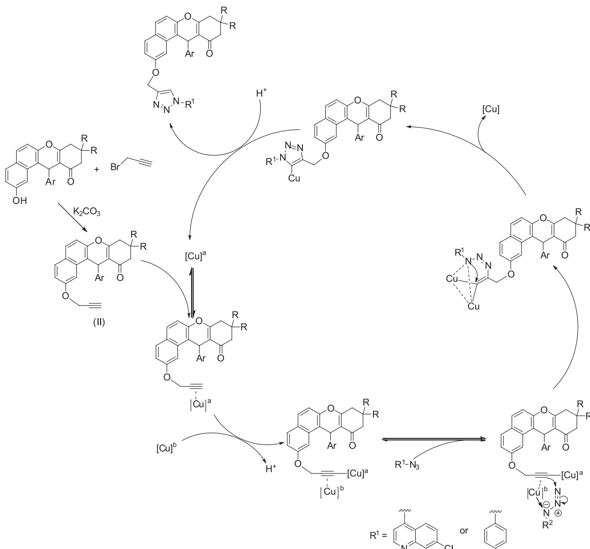
Scheme 3. Plausible reaction mechanism for synthesis of xanthene-triazole-quinoline conjugates.
