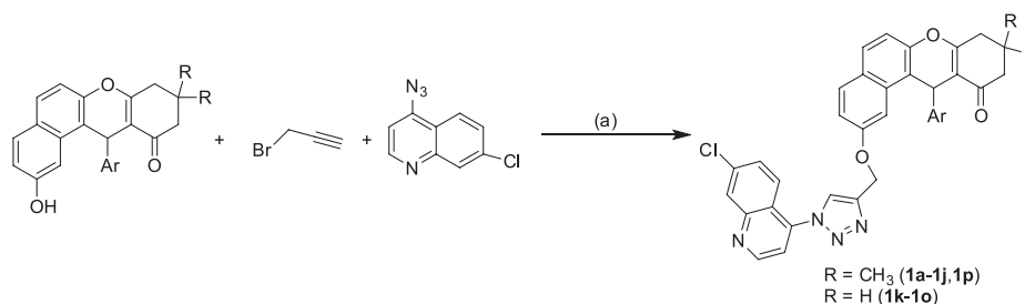
Scheme 2. Multicomponent synthesis of 2-((1-(7-chloroquinolin-4-yl)-1H-1,2,3-triazol-4-yl)methoxy)-12-aryl-8,9,10,12-tetrahydrobenzo[a]xanthen-11-one derivatives. Reagents and conditions: (a) K 2 CO 3 (1 eq.), CuSO 4 ·5H 2 O (10 mol%), sodium ascorbate (10 mol%) PEG-400, 80 °C.
