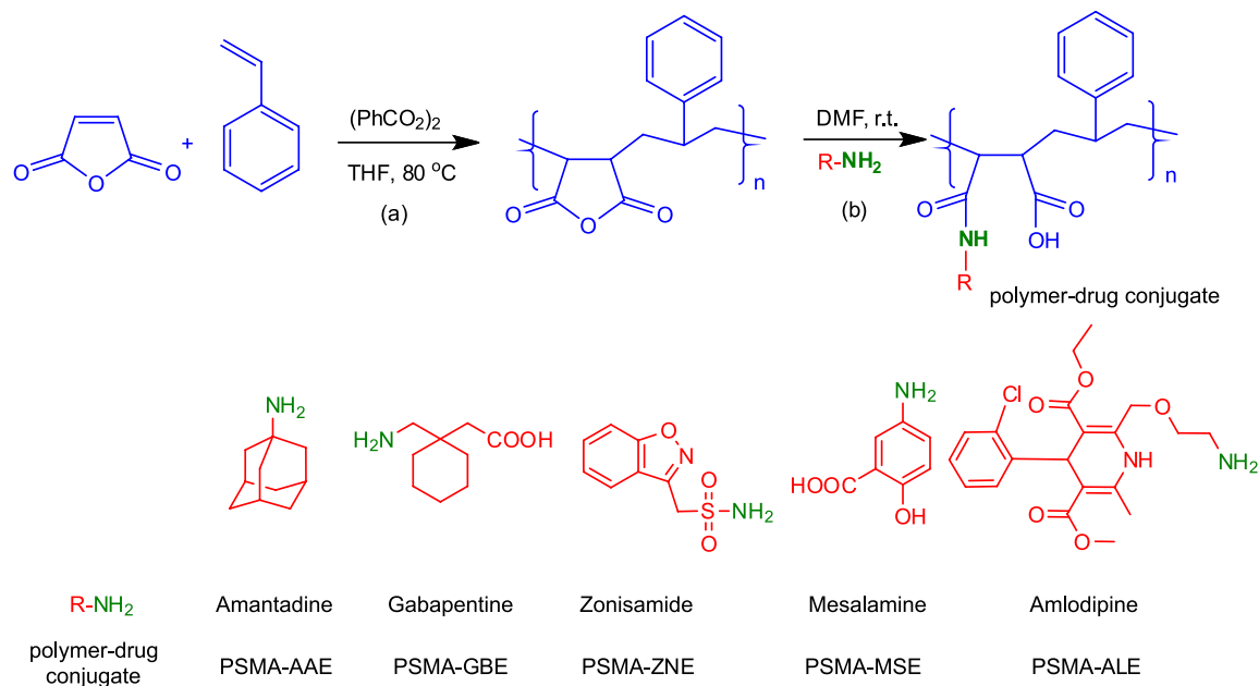
Scheme 1. General synthetic scheme: (a) copolymerization of PSMA and (b) grafting of amino drugs to PSMA.
