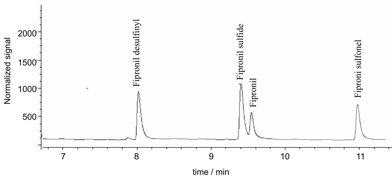
Figure S1. Chromatogram of the second point of the analytical curves containing fipronil and metabolites at the concentration of 5 \mu\text{g L}^{-1} .
