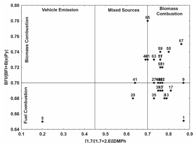
Figure 8. Cross plot of PAH diagnostic ratios. Benzo(b,k,j)fluoranthene (BFl), benzo(e)pyrene (BePy), 1,7-dimethylphenanthrene (1,7DMPH), 2,6-dimethylphenanthrene (2,6DMPH).
