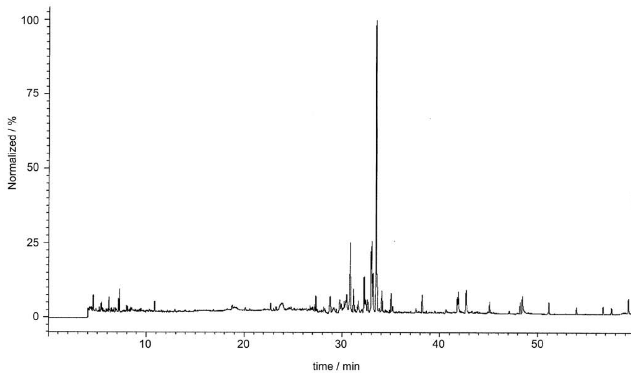
Figure S2. GC-MS chromatogram of the essential oil from fruits of Eugenia langsdorffii .
