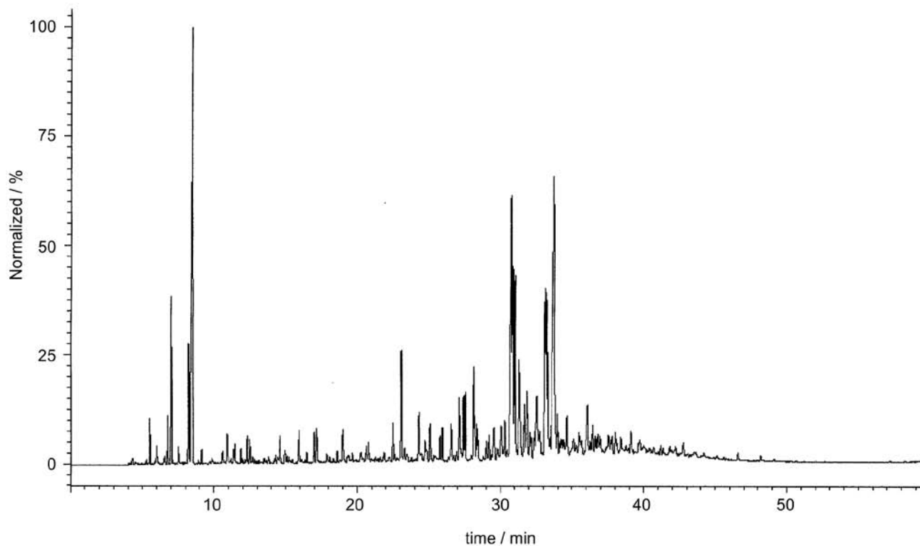
Figure S1. GC-MS chromatogram of the essential oil from leaves of Eugenia langsdorffii .
