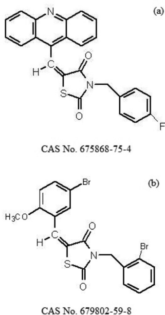
Figure 1. Structural formula of the compound (a) 2,4-thiazolidinedione, 5-(9-acridinylmethylene)-3-[(4-fluorophenyl)methyl] and (b) of the internal standard 2,4-thiazolidinedione, 5-[(5-bromo-2-methoxyphenyl)methylene]-3-[(2-bromophenyl)methyl].
