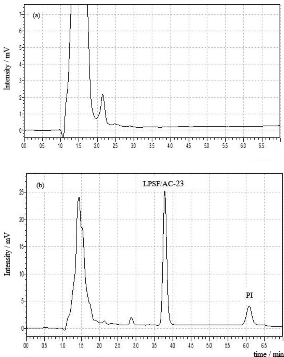
Figure 4. (a) Chromatogram of blank plasma and (b) chromatogram of the medium-quality controls sample (MQC, 5000 ng mL -1 ), using as mobile phase 5 mmol L -1 acetonitrile/methanol/phosphate buffer (55:30:15) of pH 6.0 with flow rate of 1 mL min -1 and temperature of 40 °C.
