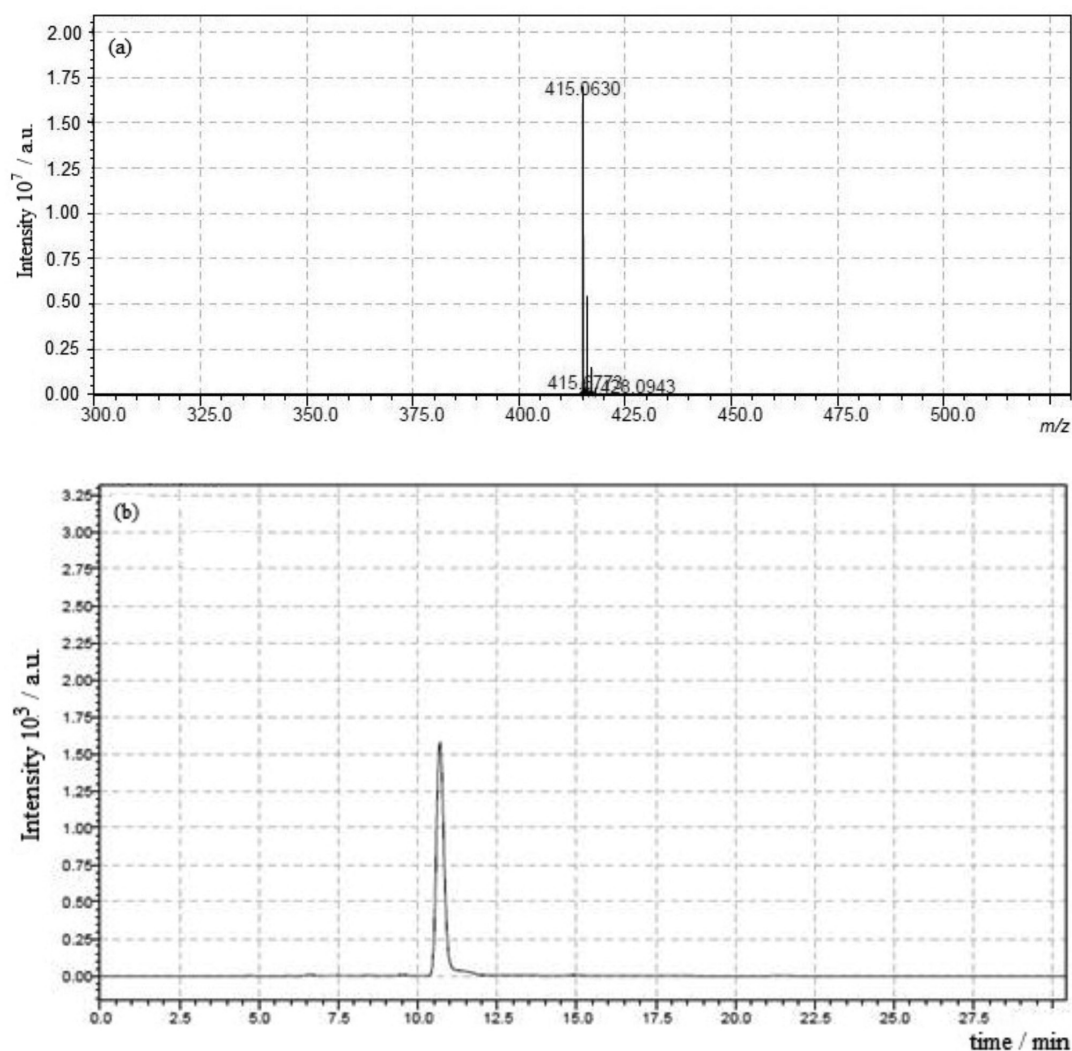
Figure 2. (a) Mass spectrum and (b) chromatogram of the sample composed of 2,4-thiazolidinedione,5-(9-acridinylmethylene)-3-[(4-fluorophenyl)methyl] at a concentration of 7000\text{ ng mL}^{-1} , obtained by ESI (negative mode) at 40^{\circ}\text{C} on a Shimadzu LC-MS-IT-TOF.
