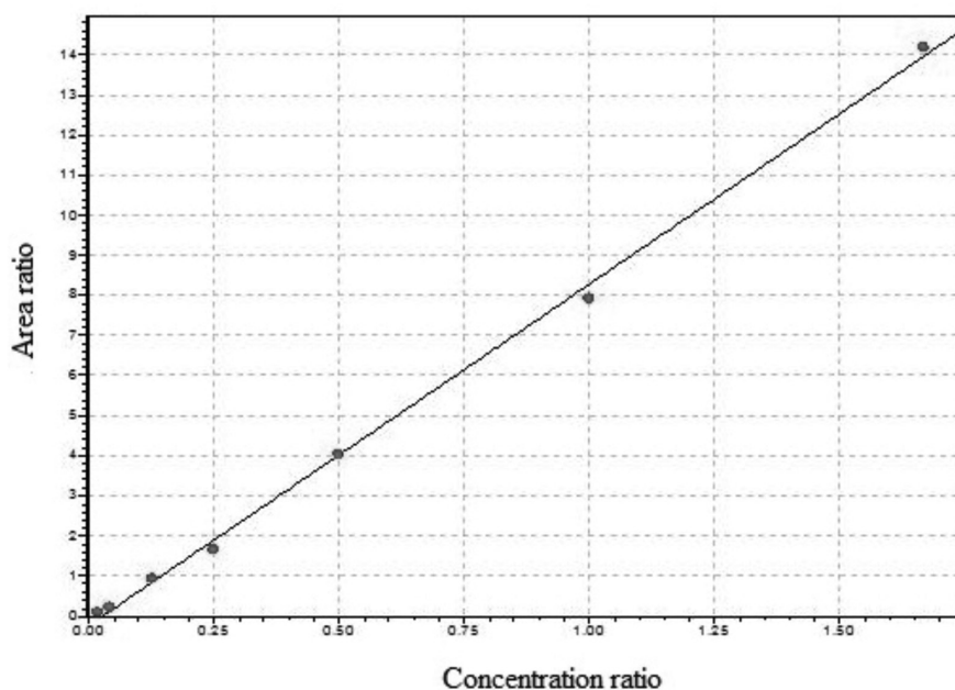
Figure 5. Average analytical curve of LPSF/AC-23. The average equation of the calibration curve was y = 7.9472x - 0.1815 ; the average of r = 0.9968 and r^2 = 0.9936 .
