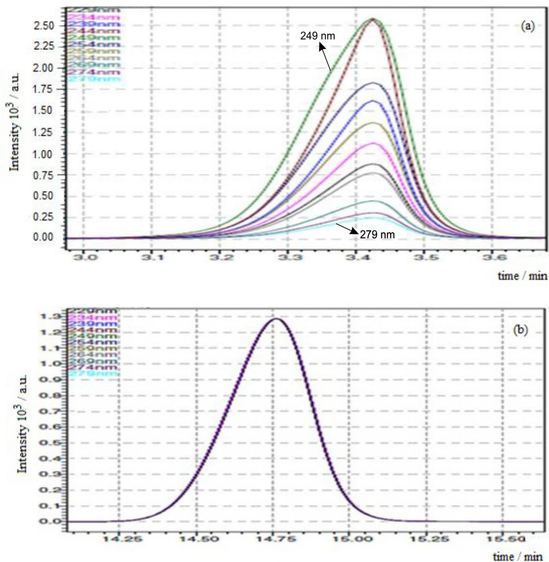
Figure 3. Chromatograms of scanning diode array detector of the (a) sample containing the compound 2,4-thiazolidinedione,5-(9-acridinylmethylene)-3-[(4-fluorophenyl)methyl] and (b) the sample containing internal standard.
