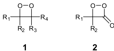
Scheme 1. General structures of 1,2-dioxetane ( 1 ) and 1,2-dioxetanone ( 2 ).
