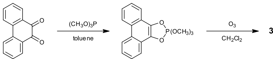
Scheme 3. Preparation of diphenoyl peroxide ( 3 ), by ozonization of the 9,10-phenanthrenequinone trimethylphosphite adduct.
