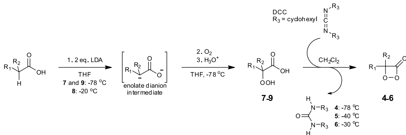
Scheme 6. General procedure for the preparation of 1,2-dioxetanones by DCC-induced cyclization of \alpha -hydroperoxyacids obtained by autoxidation of \alpha -lithio carboxylic acids.
