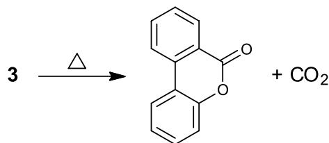
Scheme 5. Thermal decomposition of diphenoyl peroxide ( 3 ) leading to CO 2 and 6 H -benzo[ c ]chromen-6-one, a benzocoumarin derivative.
