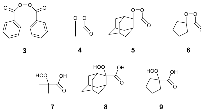
Scheme 2. Cyclic organic peroxides 3-6 prepared in the present study as well as the \alpha -hydroperoxyacid precursors 7-9 .
