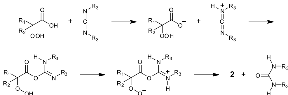
Scheme 7. Proposed mechanism for DCC-induced 1,2-dioxetanone ( 2 ) formation by dehydration/cyclization of the corresponding \alpha -hydroperoxyacids; \text{R}_3 = cyclohexyl.
