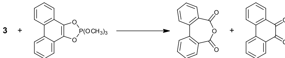
Scheme 4. Reaction of diphenoyl peroxide ( 3 ) with the trimethylphosphite adduct leading to diphenic anhydride and 9,10-phenanthrenequinone, occurring at low ozone production rates.
