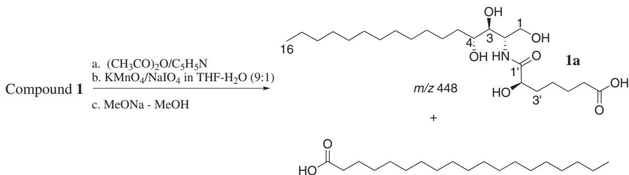
Scheme 1. Oxidative cleavage of 1 .
