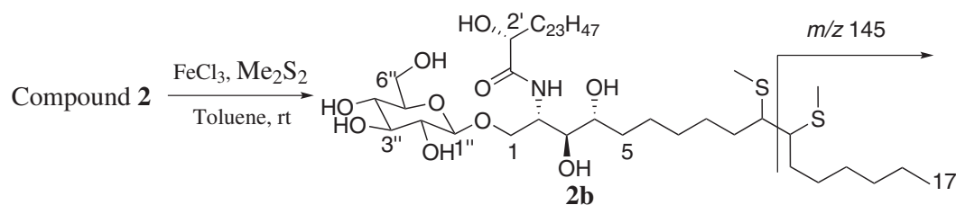
Scheme 2. Determination of double bond location by disulfenylation and MS analysis.
