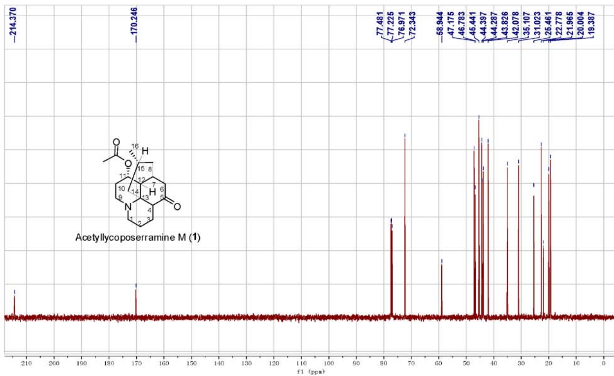
Figure S2. ^{13}\text{C} NMR spectrum of 1 .
