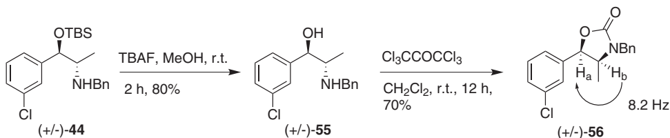
Scheme 2. Relative stereochemistry assignment of the 1,2- anti aminoalcohol derivatives.
