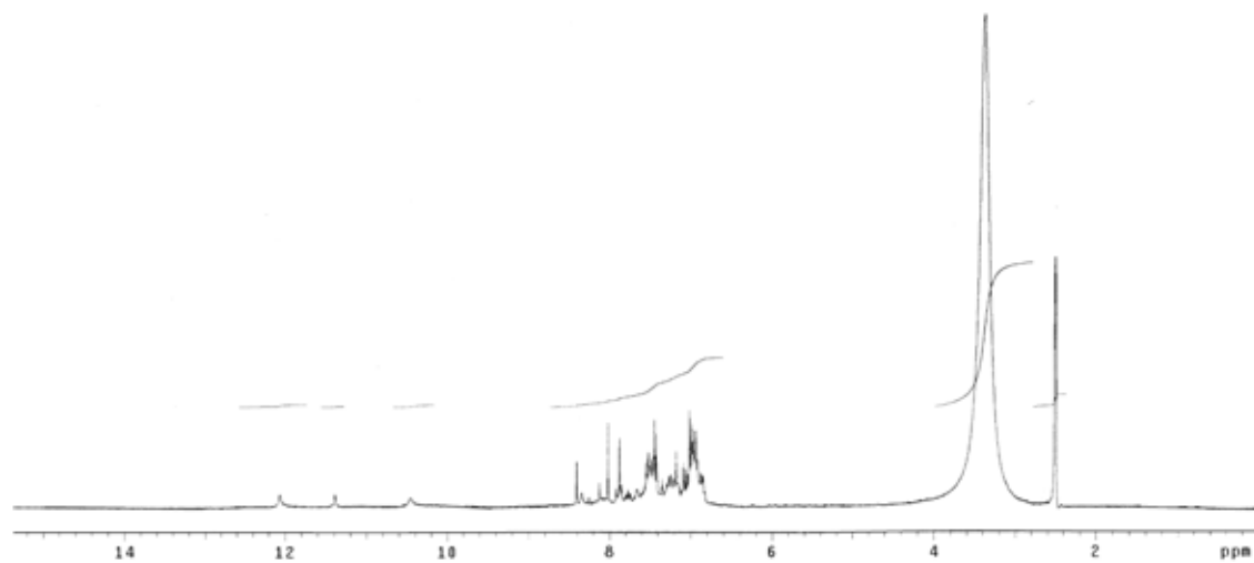
Figure S9. 1 H NMR spectrum of compound 10.
