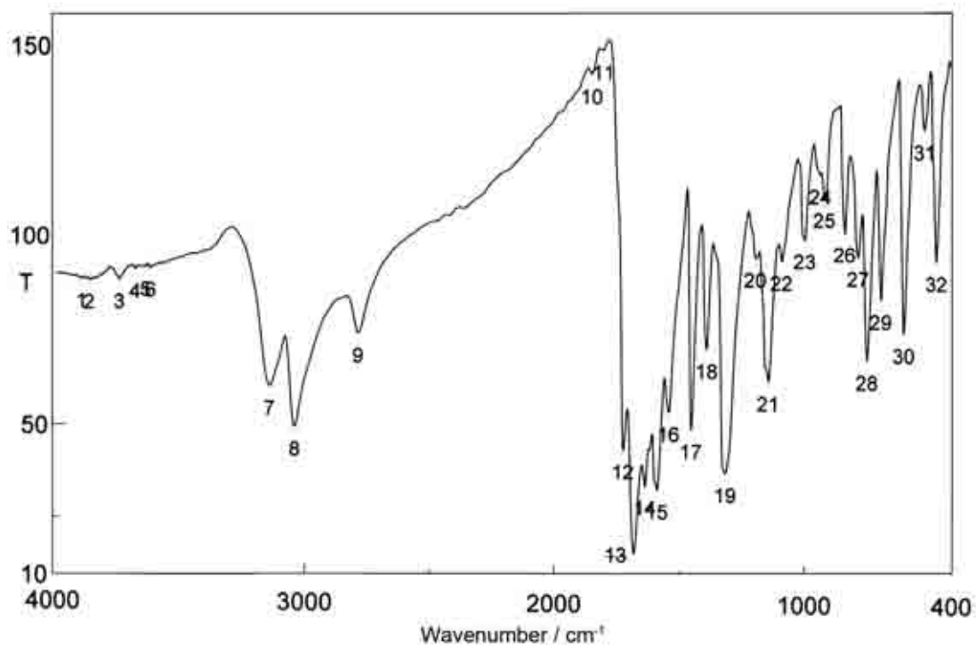
Figure S1. IR spectrum of compound 3.
