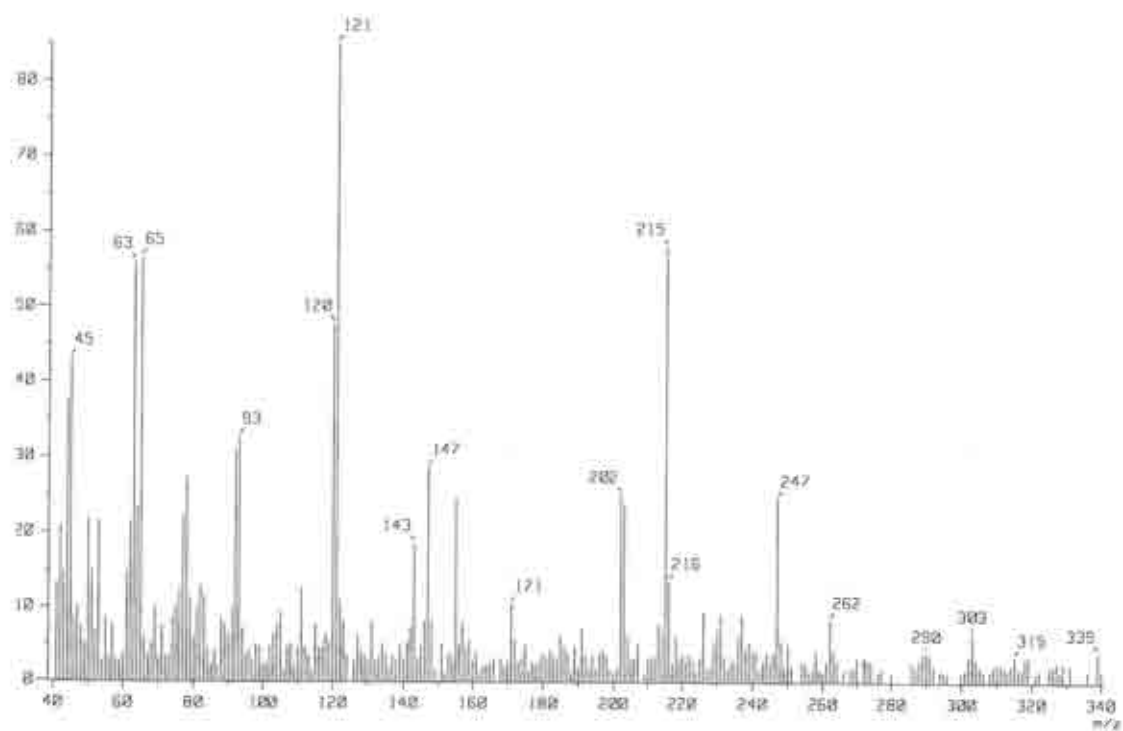
Figure S17. Mass spectrum of compound 22.
