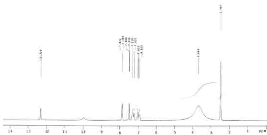
Figure S7. ^1\text{H} NMR spectrum of compound 7.
