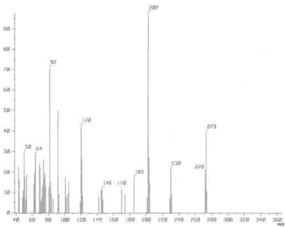
Figure S3. Mass spectrum of compound 3.
