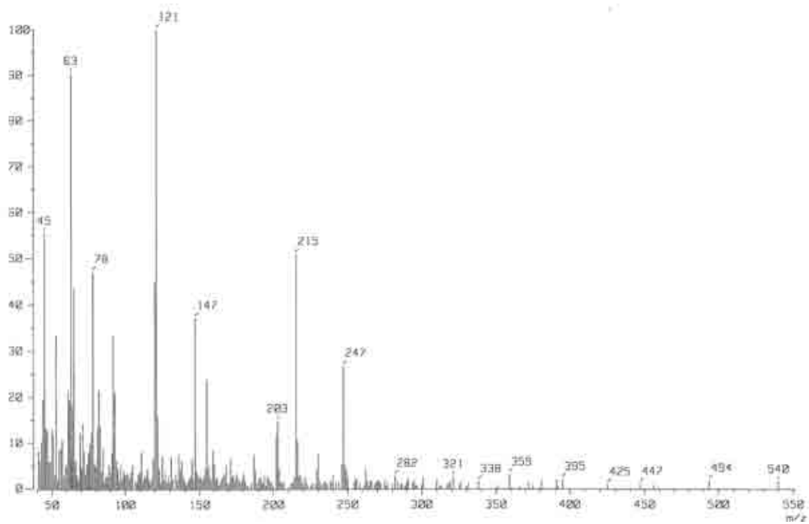
Figure S15. Mass spectrum of compound 16.
