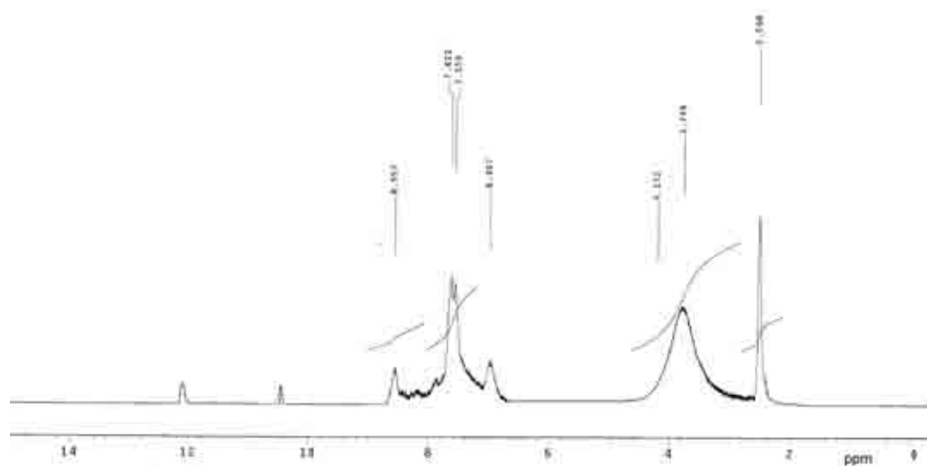
Figure S14. 1 H NMR spectrum of compound 16.
