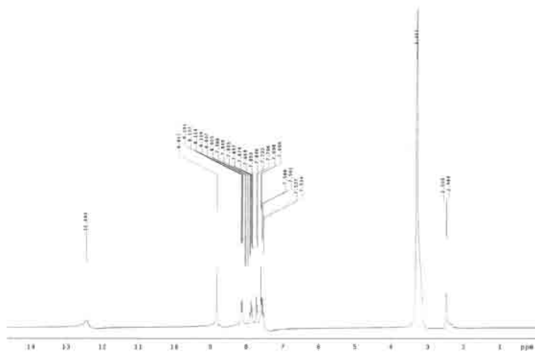
Figure S2. ^1\text{H} NMR spectrum of compound 3.
