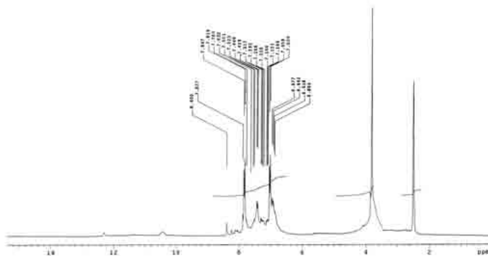
Figure S11. 1 H NMR spectrum of compound 12.
