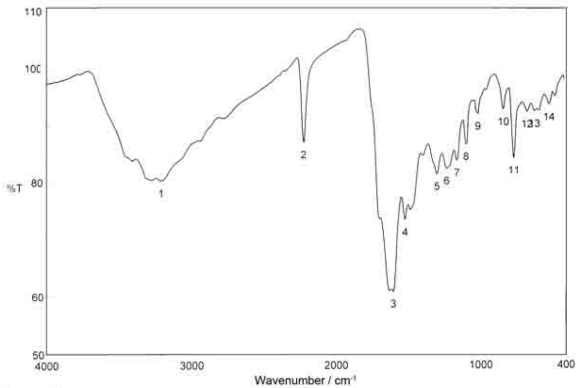
Figure S13. IR spectrum of compound 16.
