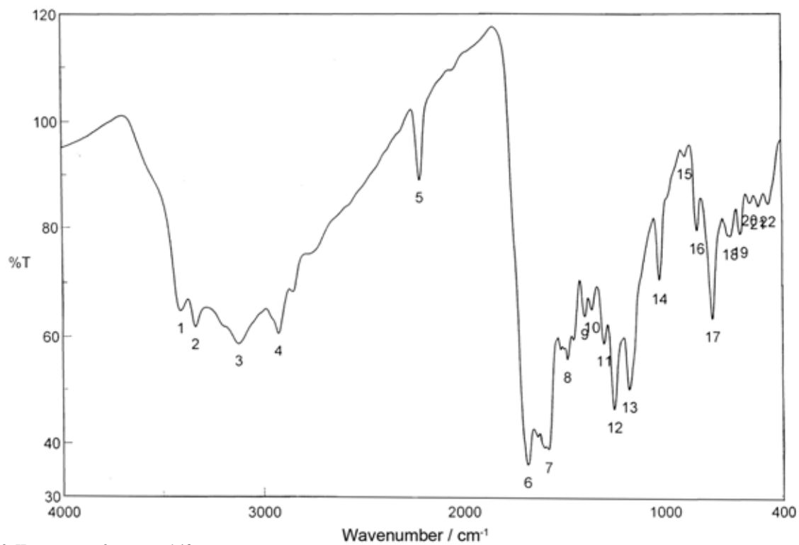
Figure S10. IR spectrum of compound 12.
