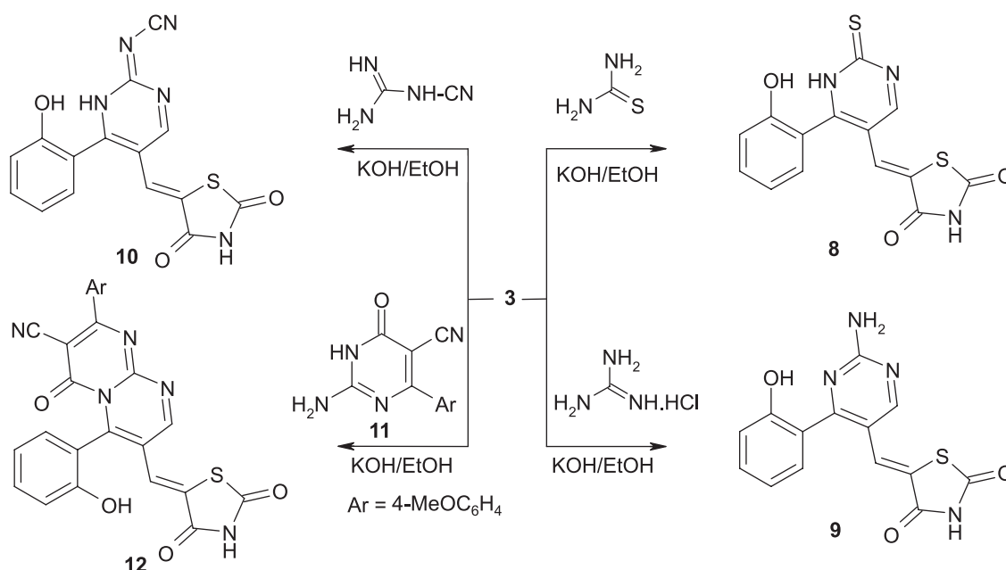
Scheme 3. Reactions of compound 3 with 1,3-bifunctional nucleophiles.
