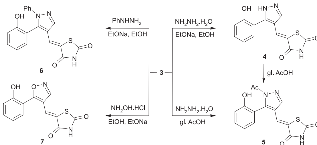
Scheme 2. Reactions of compound 3 with 1,2-bifunctional nucleophiles.
