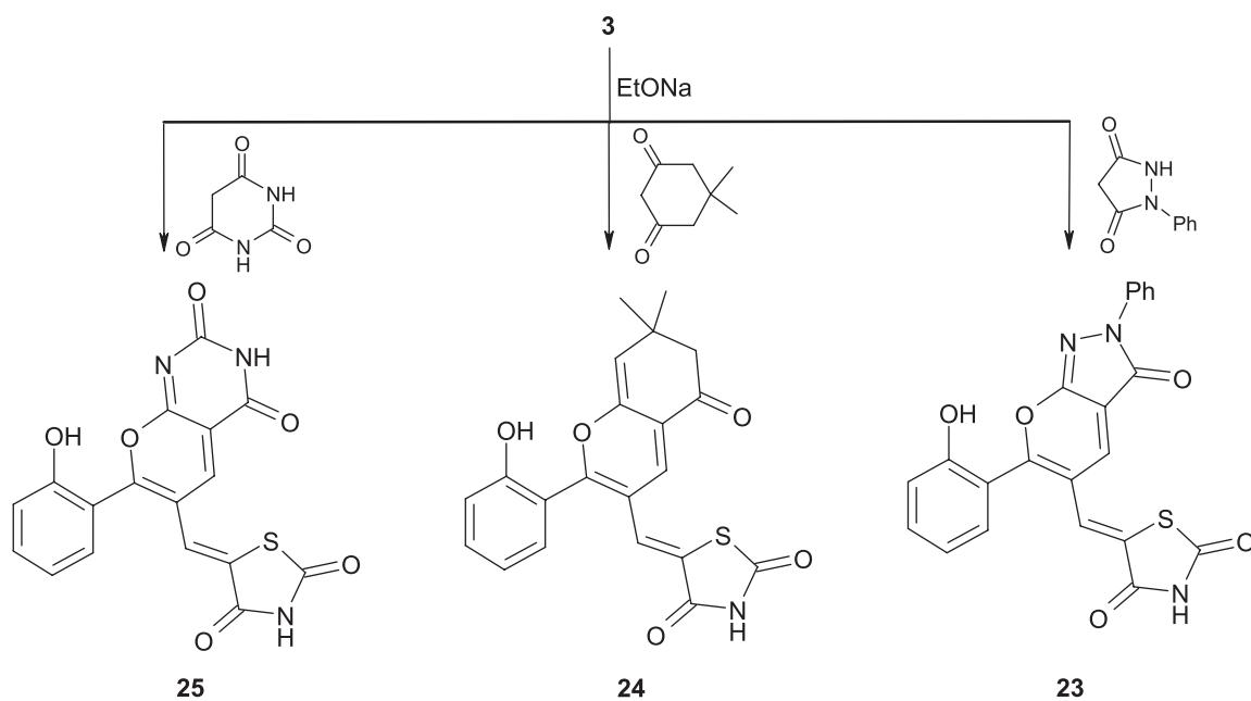
Scheme 6. Formation of 1,3-thiazolidinedione derivatives 23-25 .
