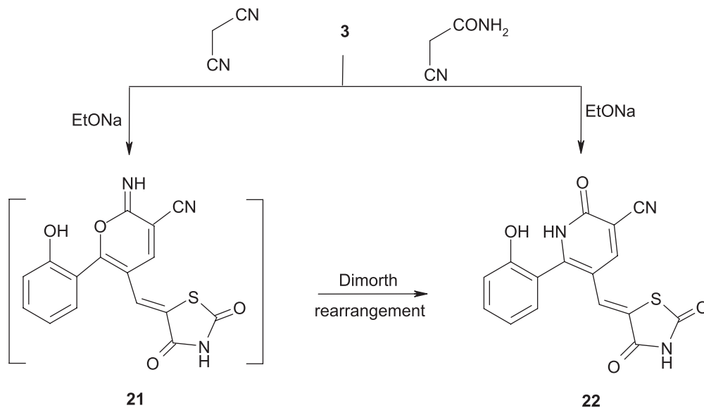
Scheme 5. Reactions of compound 3 with malononitrile and cyanoacetamide.
