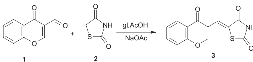
Scheme 1. Formation of chromenylthiazolidine-2,4-dione 3 .
