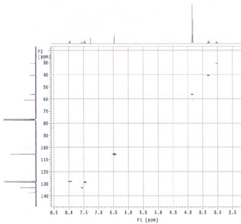
Figure S4. HETCOR spectrum ( \text{CDCl}_3 ) of compound 5 .
