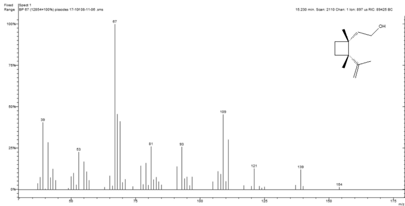
Figure S2. Mass spectrum of grandisol.
