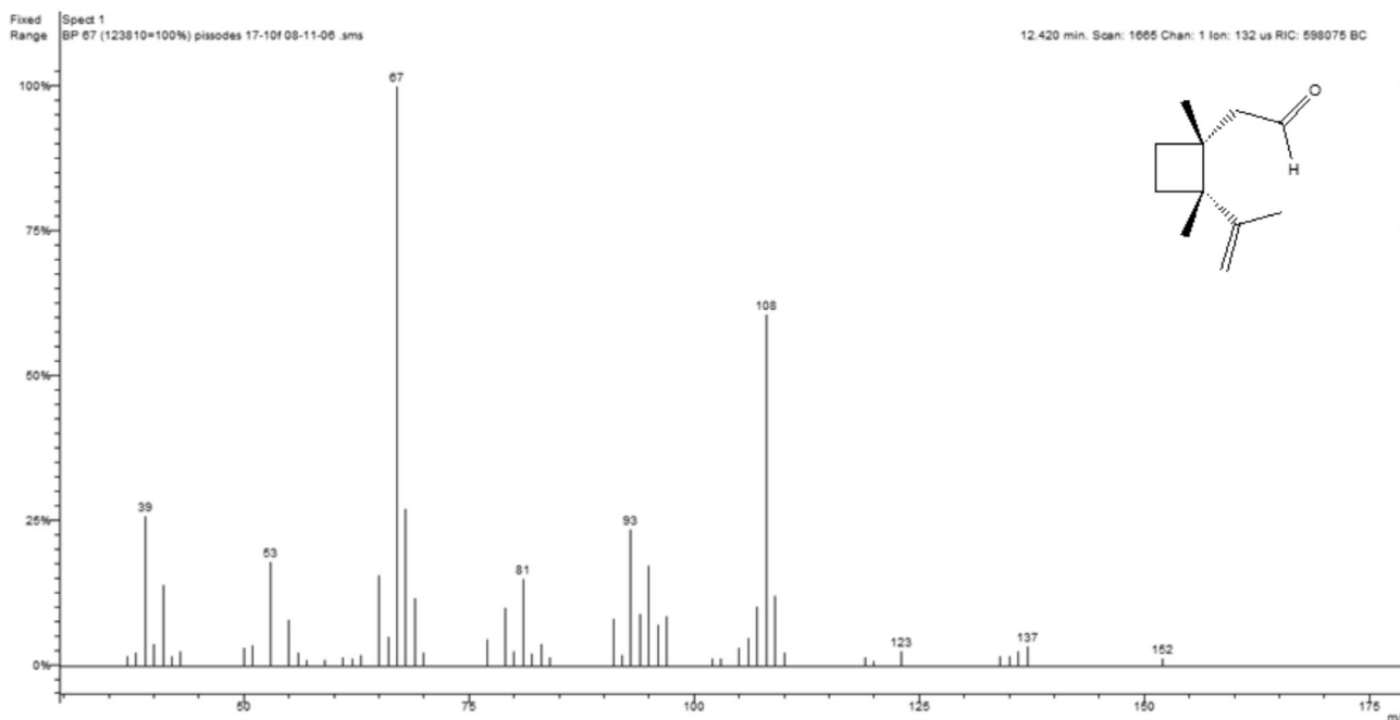
Figure S1. Mass spectrum of grandisal.
