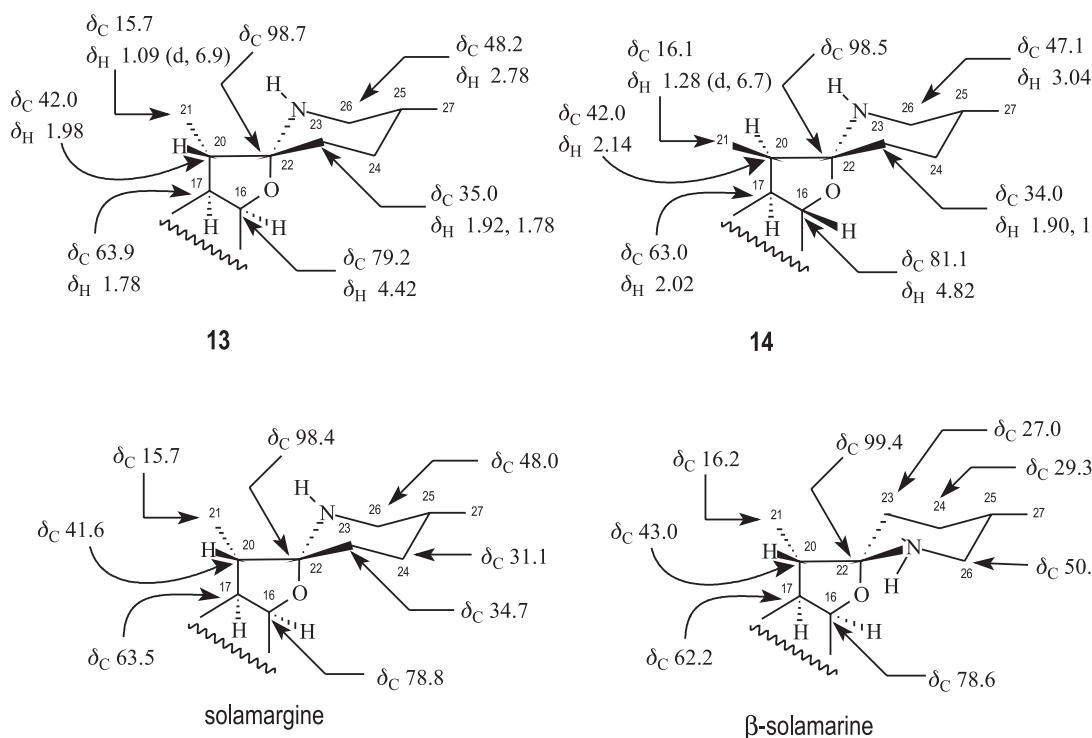
Figure 1. Comparative analysis of the chemical shifts corresponding to the hydrogen ( \delta_H ) and carbon ( \delta_C ) atoms CH-16, CH-17, CH-20, CH_3 -21, C-22, CH_2 -23 and CH_2 -26 of 13 and 14 , including comparison of the \delta_C these carbon atoms and of the CH_2 -24 to reveal the structural distinction between solamargine and \beta -solamargine.
