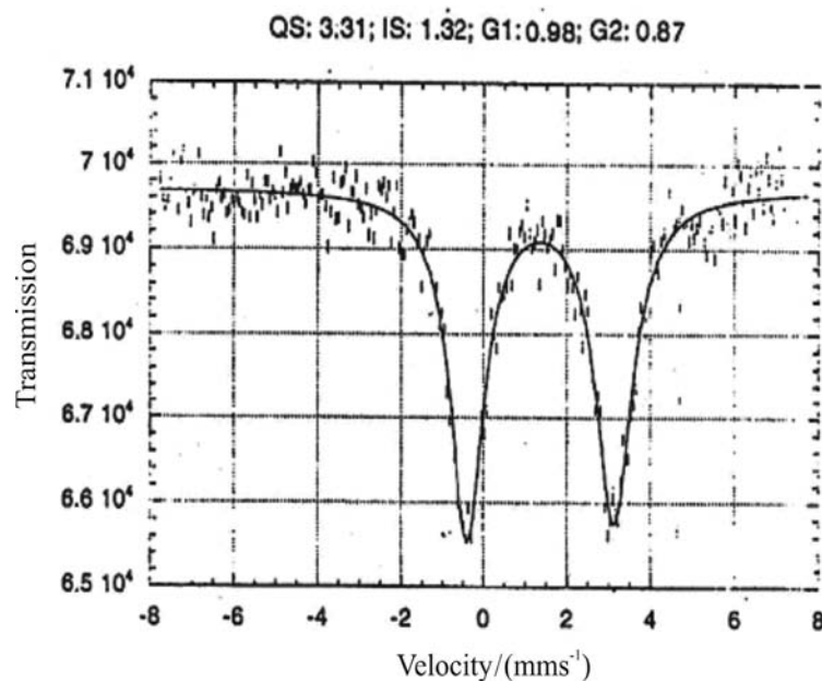
Figure S2. 119m Sn Mössbauer Spectrum of compound 1.
