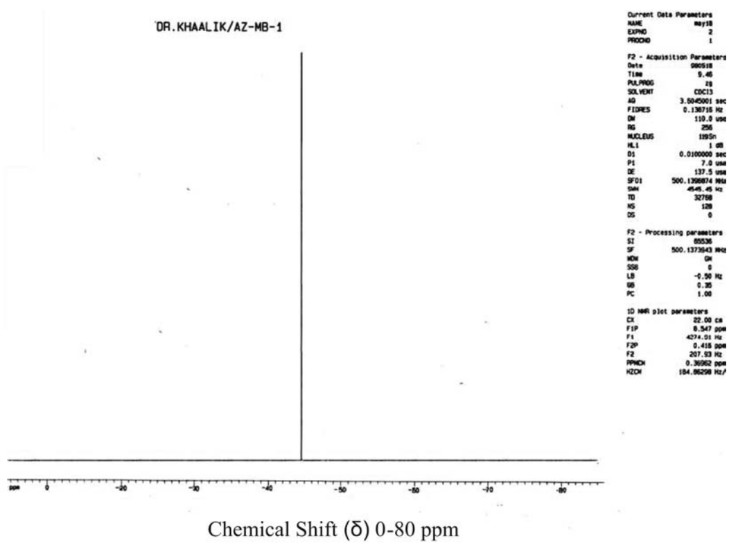
Figure S5. ^{119}\text{Sn} NMR Spectrum of compound 6.
