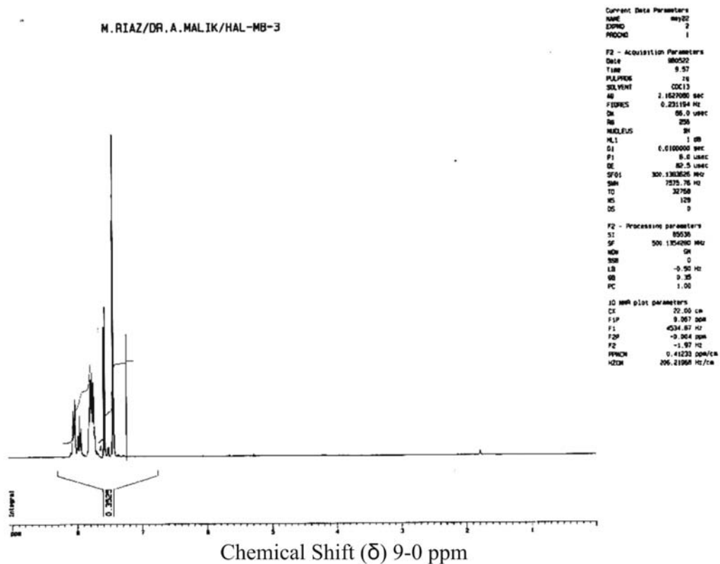
Figure S3. ^1\text{H} NMR Spectrum of compound 1.
