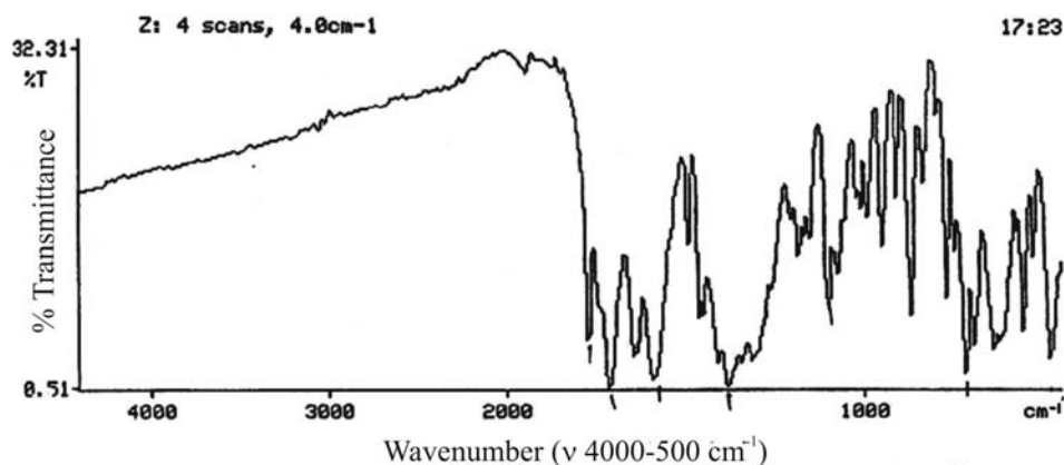
Figure S1. FT IR Spectrum of compound 1.
