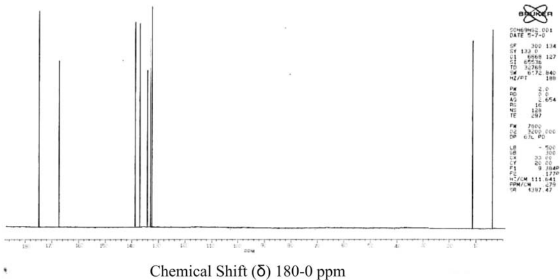
Figure S4. ^{13}\text{C} NMR Spectrum of compound 2.
