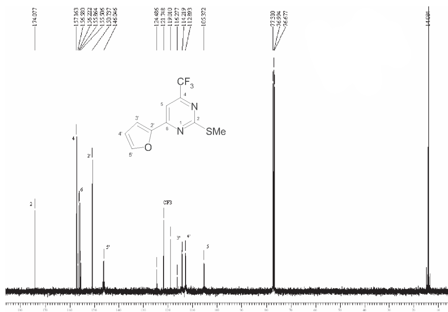
Figure S23. ^{13}\text{C} NMR spectrum of the 6-(2-furyl)-2-methyl-4-trifluoromethylpyrimidine 7a , \text{CDCl}_3 .
