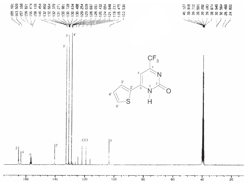
Figure S4. 13 C NMR spectrum of the 6-(2-thienyl)-4-trifluoromethyl-1H-pyrimidin-2-one (2b), DMSO- d 6 .
