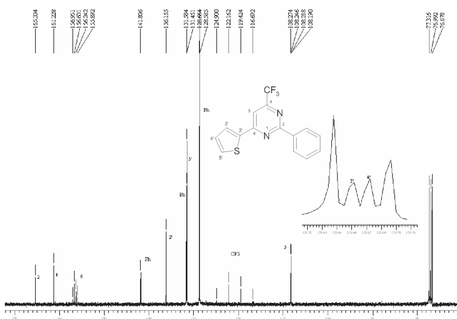
Figure S13. ^{13}\text{C} NMR spectrum of the 2-phenyl-6-(2-thienyl)-4-trifluoromethylpyrimidine 4b , CDCl 3 .
