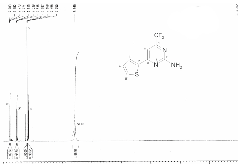
Figure S16. 1 H NMR spectrum of the 2-amino-6-(2-thienyl)-4-trifluoromethylpyrimidine 5b , CDCl 3 .
