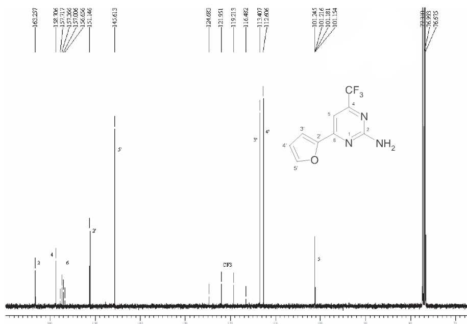
Figure S15. 13 C [H] NMR spectrum of the 2-amino-6-(2-furyl)-4-trifluoromethylpyrimidine 5a , CDCl 3 .
