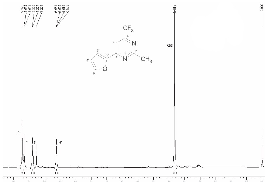
Figure S5. 1 H NMR spectrum of the 6-(2-furyl)-2-methyl-4-trifluoromethylpyrimidine (3a), CDCl 3 .
