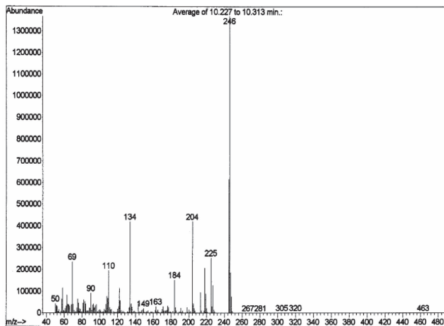
Figure S27. MS of 6-(2-thienyl)-4-trifluoromethyl-1H-pyrimidin-2-one (2b).
