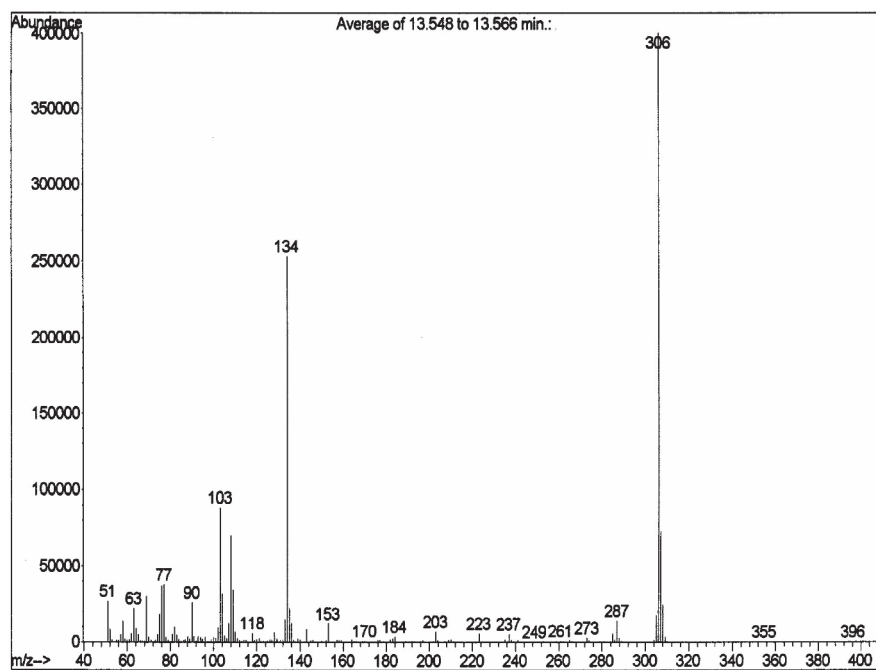
Figure S31. MS of 2-phenyl-6-(2-thienyl)-4-trifluoromethylpyrimidine (4b).
