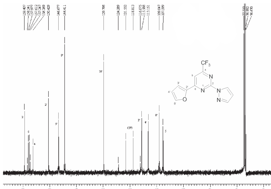
Figure S19. ^{13}\text{C} NMR spectrum of 6-(2-furyl)-2-(1 H -pyrazol-1-yl)-4-trifluoromethyl-pyrimidine 6a , \text{CDCl}_3 .
