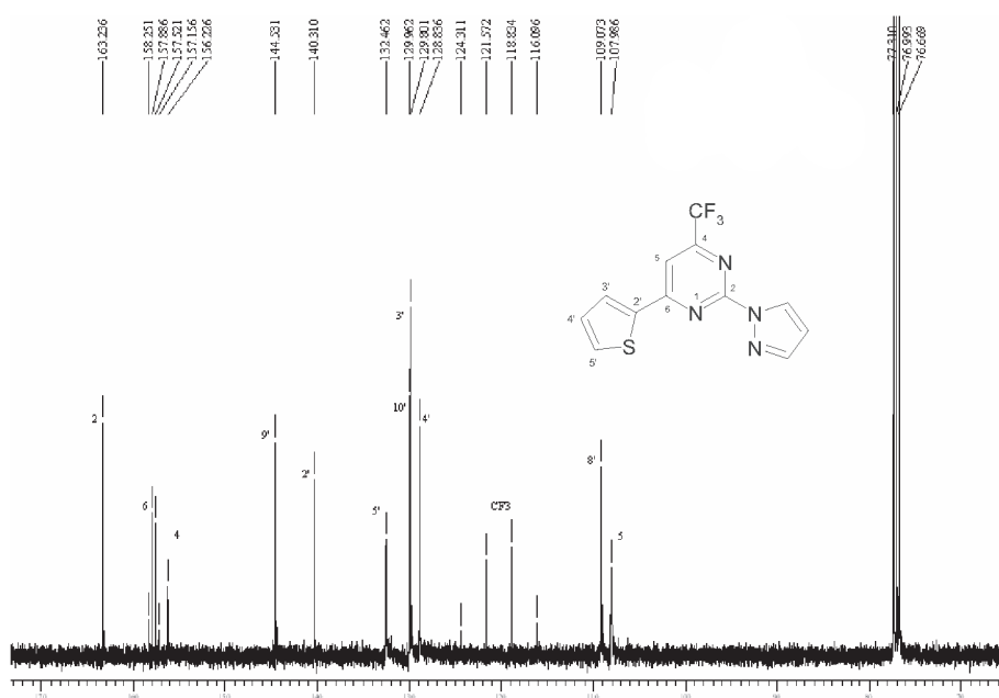
Figure S21. 13 C NMR spectrum of the 2-(1H-pyrazol-1-yl)-6-(2-thienyl)-4-trifluoromethylpyrimidine 6b , CDCl 3 .
