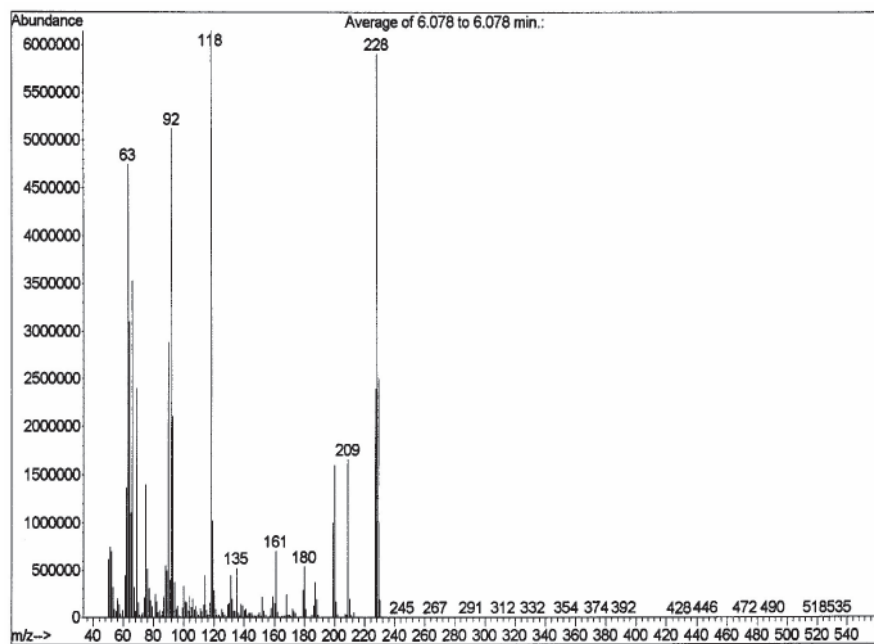
Figure S28. MS of 6-(2-furyl)-2-methyl-4-trifluoromethylpyrimidine (3a).
