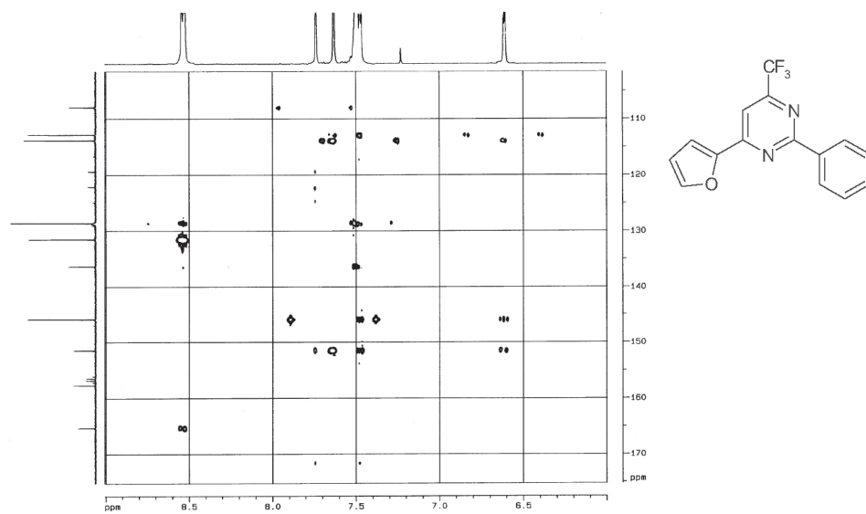
Figure S11. HMBC spectrum of the 6-(2-furyl)-2-phenyl-4-trifluoromethylpyrimidine 3b , \text{CDCl}_3 .
