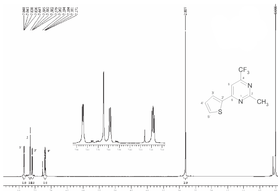
Figure S7. 1 H NMR spectrum of the 2-methyl-6-(2-thienyl)-4-trifluoromethylpyrimidine ( 3b ), CDCl 3 .
