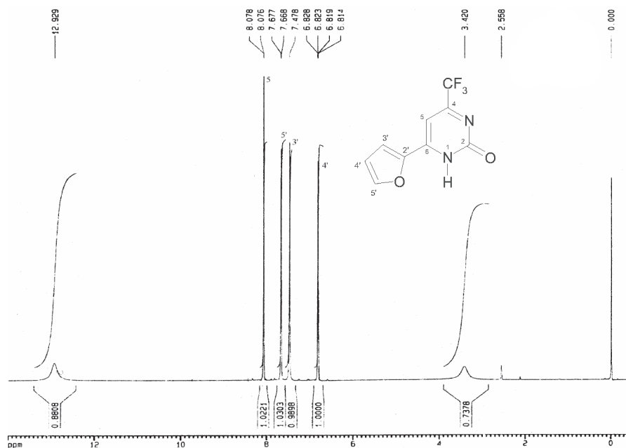
Figure S1. 1 H NMR spectrum of the 6-(2-furyl)-4-trifluoromethyl-1H-pyrimidin-2-one (2a), DMSO-d 6 .
