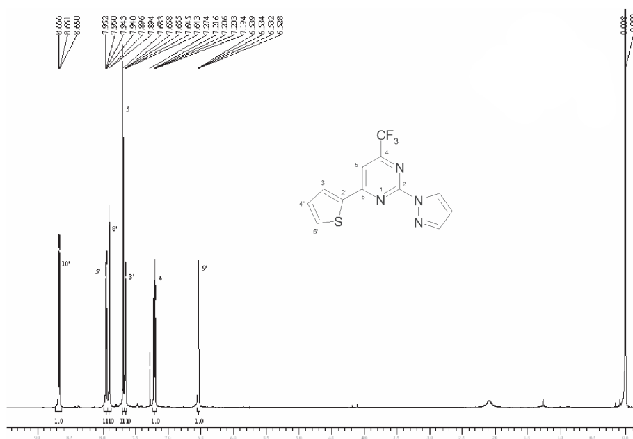
Figure S20. 1 H NMR spectrum of the 2-(1H-pyrazol-1-yl)-6-(2-thienyl)-4-trifluoromethylpyrimidine 6b , CDCl 3 .
