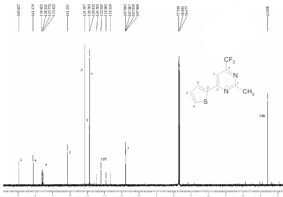
Figure S8. ^{13}\text{C} [H] NMR spectrum of the 6-(2-thienyl)-2-methyl-4-trifluoromethylpyrimidine 3b , \text{CDCl}_3 .
