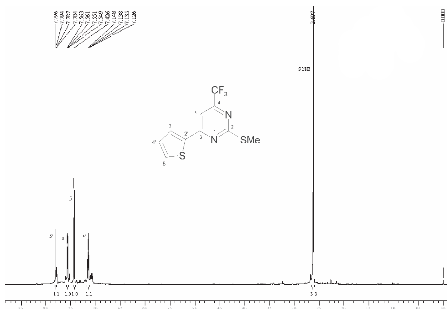
Figure S24. 1 H NMR spectrum of the 6-(2-thienyl)-2-methyl-4-trifluoromethylpyrimidine 7b , CDCl 3 .
