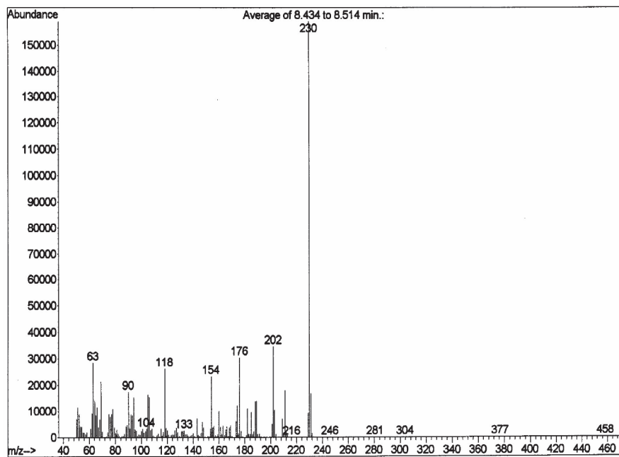
Figure S26. MS of 6-(2-furyl)-4-trifluoromethyl-1H-pyrimidin-2-one (2a).
