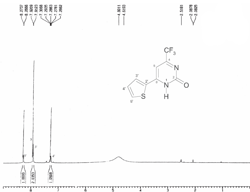
Figure S3. ^1\text{H} NMR spectrum of the 6-(2-thienyl)-4-trifluoromethyl-1 H -pyrimidin-2-one ( 2b ), \text{DMSO-}d_6 .
