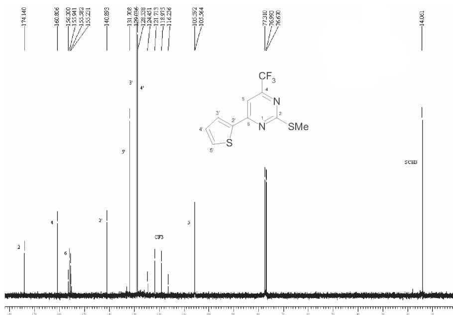
Figure S25. 13 C NMR spectrum of the 6-(2-thienyl)-2-methyl-4-trifluoromethylpyrimidine 7b , CDCl 3 .
