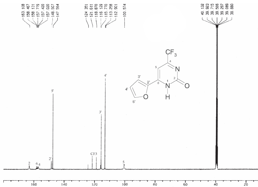
Figure S2. ^{13}\text{C}\{^1\text{H}\} NMR spectrum of the 6-(2-furyl)-4-trifluoromethyl-1 H -pyrimidin-2-one ( 2a ), \text{DMSO-}d_6 .
