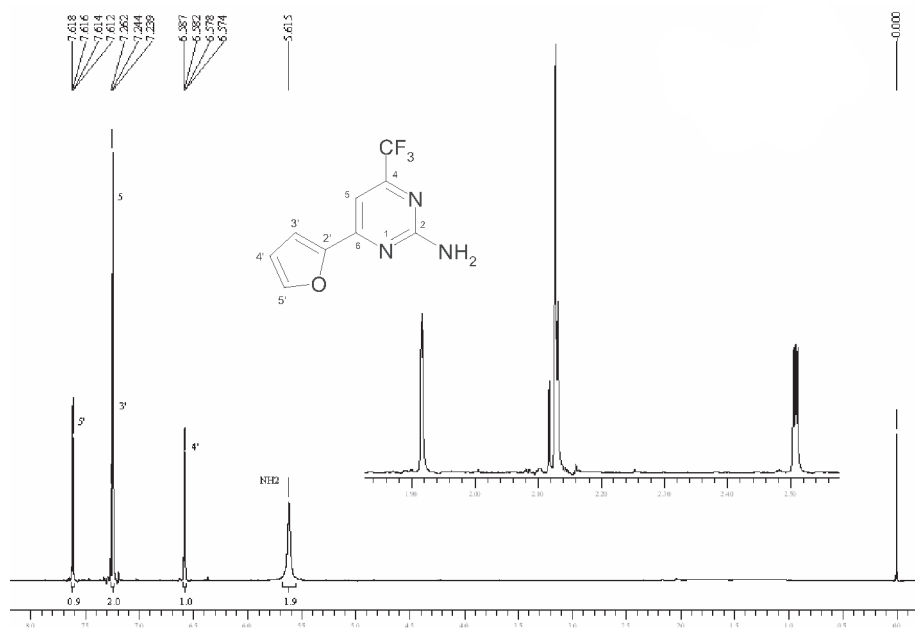
Figure S14. 1 H NMR spectrum of the 2-amino-6-(2-furyl)-4-trifluoromethylpyrimidine 5a , CDCl 3 .
