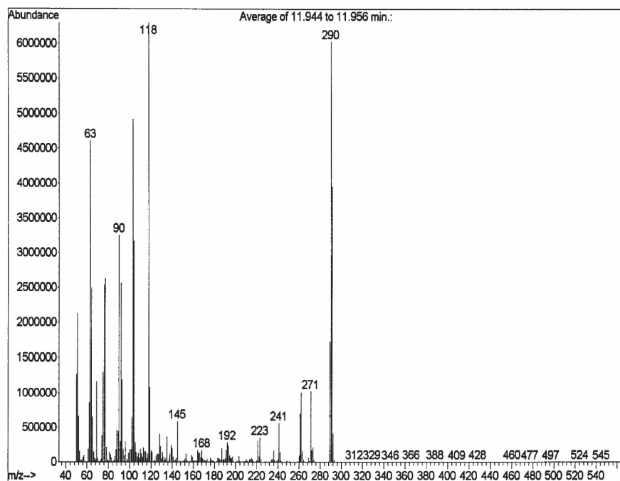
Figure S30. MS of 6-(2-furyl)-2-phenyl-4-trifluoromethylpyrimidine (4a).
