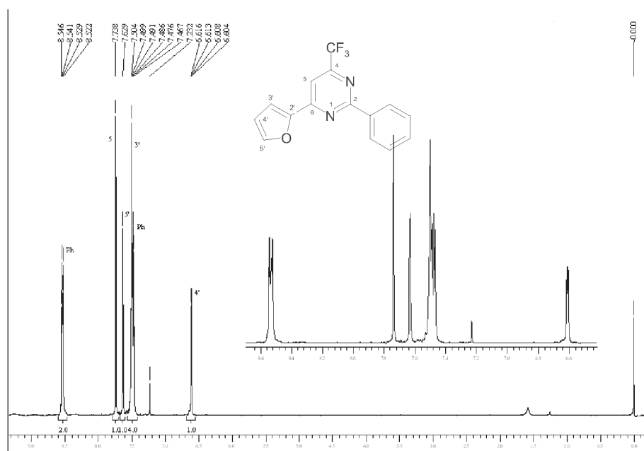
Figure S9. ^1\text{H} NMR spectrum of the 6-(2-furyl)-2-phenyl-4-trifluoromethylpyrimidine 4a , \text{CDCl}_3 .
