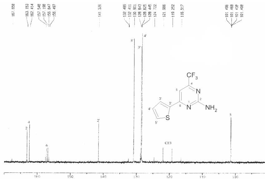
Figure S17. 13 C NMR spectrum of the 2-amino-6-(2-thienyl)-4-trifluoromethylpyrimidine 5b , CDCl 3 .
