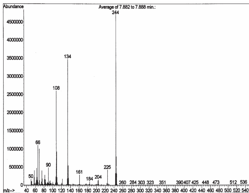
Figure S29. MS of 2-methyl-6-(2-thienyl)-4-trifluoromethylpyrimidine (3b).
