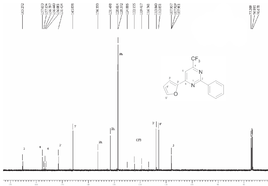
Figure S10. ^{13}\text{C} NMR spectrum of the 6-(2-furyl)-2-phenyl-4-trifluoromethylpyrimidine 4a , \text{CDCl}_3 .
