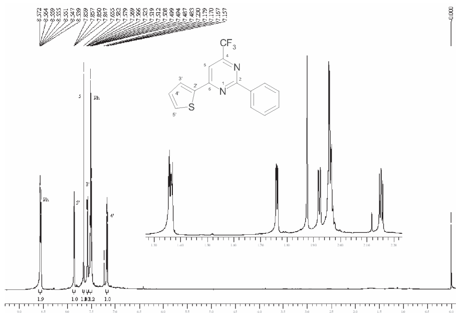
Figure S12. ^1\text{H} NMR spectrum of the 2-phenyl-6-(2-thienyl)-4-trifluoromethylpyrimidine 4b , CDCl 3 .
