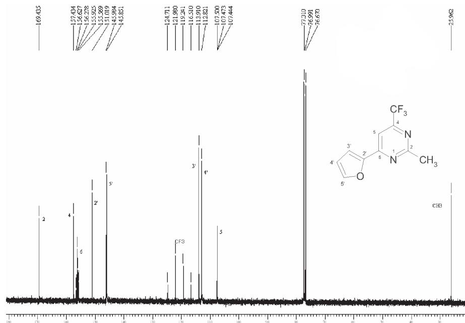
Figure S6. 13 C NMR spectrum of the 6-(2-furyl)-2-methyl-4-trifluoromethylpyrimidine ( 3a ), CDCl 3 .
