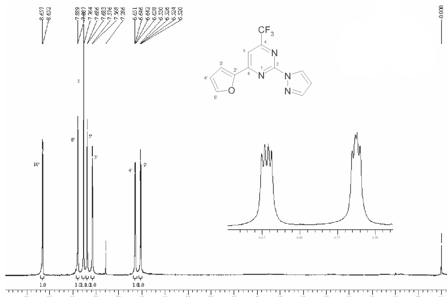
Figure S18. ^1\text{H} NMR spectrum of the 6-(2-furyl)-2-(1 H -pyrazol-1-yl)-4-trifluoromethyl-pyrimidine 6a , \text{CDCl}_3 .
