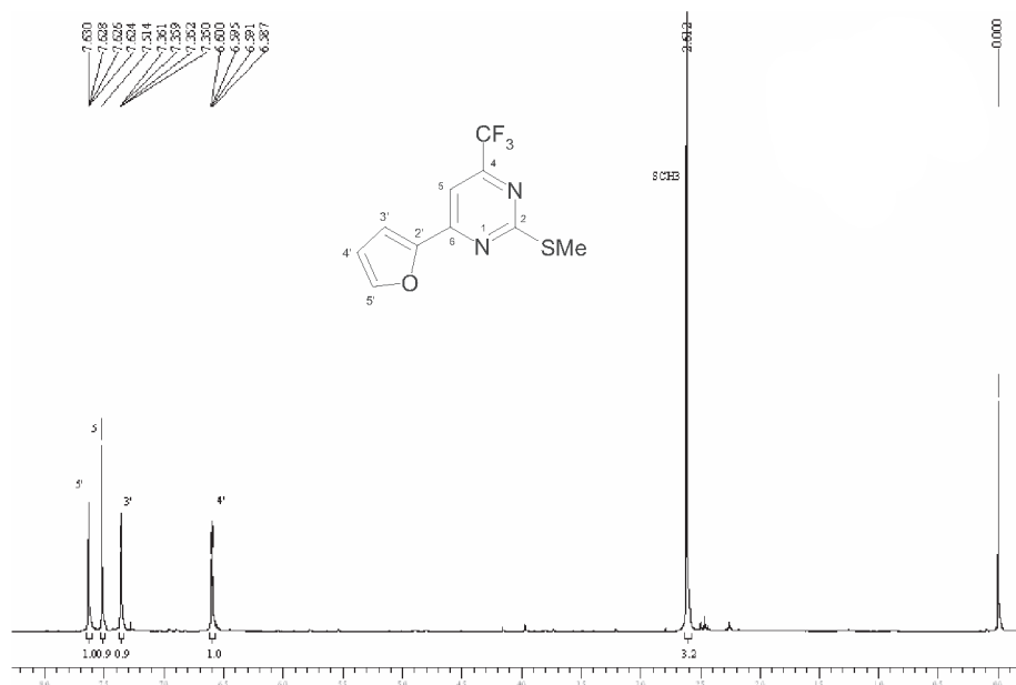
Figure S22. ^1\text{H} NMR spectrum of the 6-(2-furyl)-2-methyl-4-trifluoromethylpyrimidine 7a , \text{CDCl}_3 .
