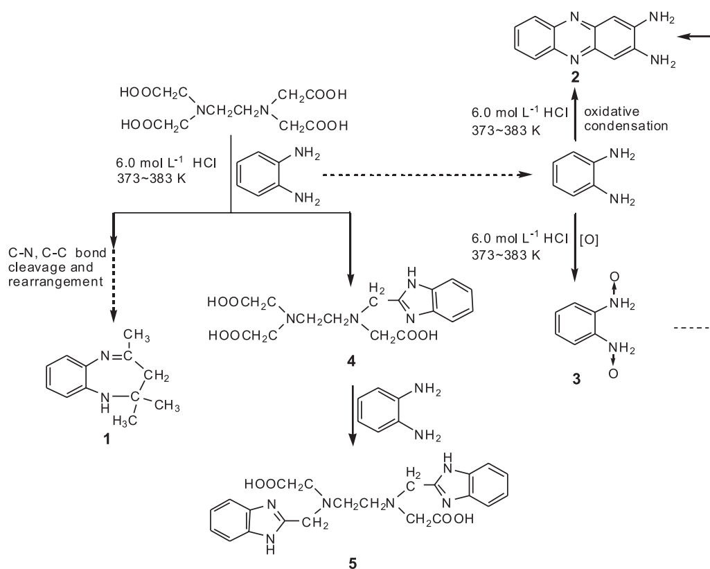
Figure 4. Thermal decomposition pathway proposed for EDTA in the presence of o -PDA in strong acidic solution at 373-383 K.
