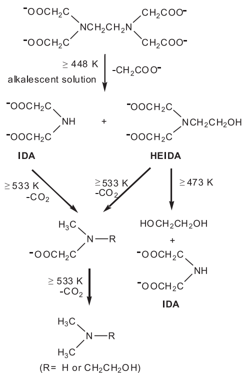
Figure 1. Different routes proposed for the decomposition of EDTA with temperature changes.
