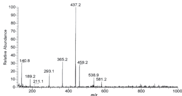
Figure 2. ES-MS spectrum detected with the reacting solution of EDTA and o -PDA in the 6 mol \text{L}^{-1} hydrochloric acid at 373–383 K (40 h) (positive ion mode). Attribution: 140.8, 1,2-phenylenediamine- N,N -dioxide; 189.2, 2,2,4-trimethyl-3H-5-hydro-1,5-benzodiazepine; 212.3, 2,3-diaminophenazine; 293.0, EDTA; 365.2, N -2-benzimidazolyl methyl-1,2-ethanediamine-trisacetic acid; 437.2, N,N' -bis(2-benzimidazolylmethyl)-1,2-ethanediamine-bisacetic acid; 459.3, N,N' -bis(2-benzimidazolylmethyl)-1,2-ethanediamine-bisacetic acid monosodium salt; 581.2, EDTB.
