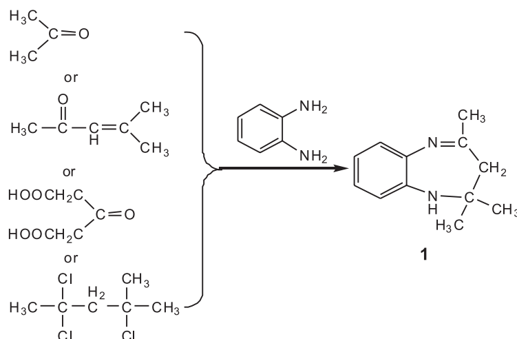
Figure 5. The known materials or intermediates for synthesis of 2,2,4-trimethyl-3H-5-hydro-1,5-benzodiazepine under different conditions.
