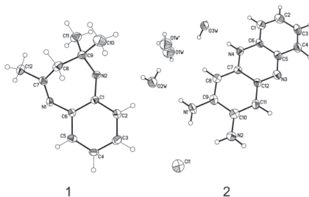
Figure 3. Crystal structures of 2,2,4-trimethyl-3H-5-hydro-1,5-benzodiazepine ( 1 ) and 2,3-diamino-5-hydrophenazinium chloride tris-hydrate ( 2 ). Selected crystal data for 1 : a = 12.210(2) Å, b = 7.3120(15) Å, c = 11.977(2) Å; \text{N1-C6} 1.406(7) Å, \text{N1-C7} 1.293(8) Å, \text{N2-C1} 1.401(7) Å, \text{N2-C9} 1.480(7) Å, \text{C7-C8} 1.499(9) Å, \text{C8-C9} 1.503(8) Å; \text{N1-C6-C1} 124.8(5)°, \text{N1-C7-C8} 123.3(5)°, \text{N2-C1-C6} 121.8(5)°, \text{N2-C9-C8} 109.1(5)°, \text{C7-C8-C9} 114.0(5)°. Selected crystal data for 2 : a = 6.8000(14) Å, b = 9.902(2) Å, c = 11.235(2) Å, \alpha = 74.49(3)^\circ , \beta = 78.26(3)^\circ , \gamma = 84.77(3)^\circ ; \text{N1-C9} 1.331(6) Å, \text{N2-C10} 1.331(7) Å; \text{N1-C9-C10} 119.7(5)°, \text{N2-C10-C9} 117.9(5)°.
