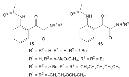
Figure 3. Structures of phenylglyoxamides ( 15 ) and mandelamides ( 16 ).
