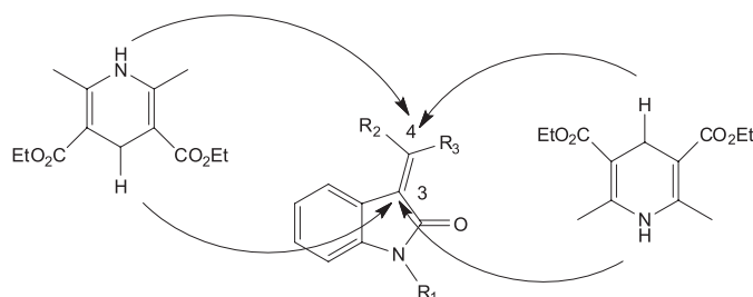
Figure 8. Representation of the hydride and proton transfers upon the reduction of methylenoxindole derivatives.
