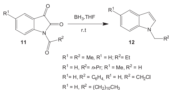
Scheme 4. Reaction conditions for the preparation of N -alkylindoles.
