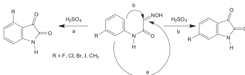
Scheme 18. Pathway of (a) formation of 4-substituted-isatins, (b) formation of 6-substituted-isatins.
