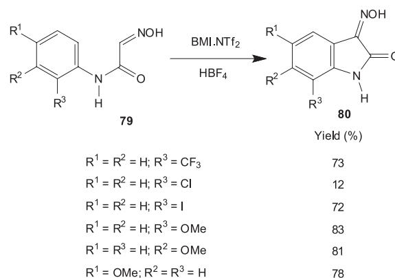
Scheme 17. Cyclisation reactions using BMLNTf 2 and HBF 4 .
