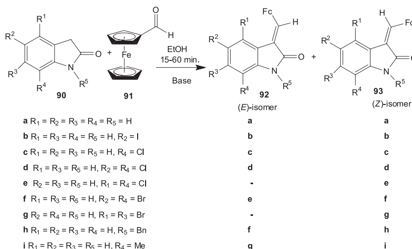
Scheme 20. Synthesis of ferrocenyl oxindoles.
