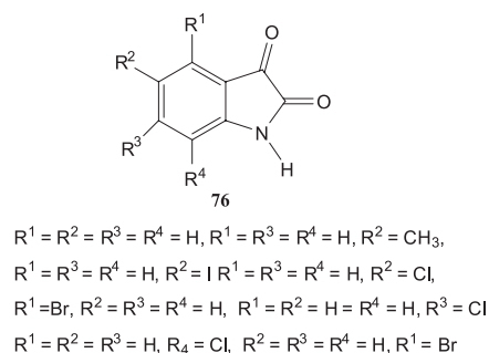
Figure 10. Structures of isatin and aromatic ring substituted derivatives.
