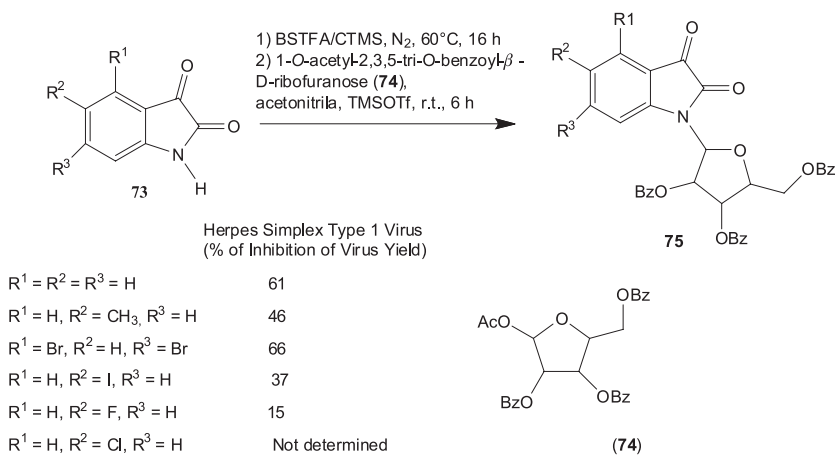
Scheme 15. Synthetic route for the preparation of isatin nucleosides ( 75 ) and the corresponding HSV-1 inhibition percentages.
