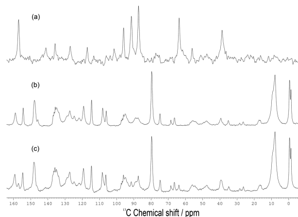
Figure 6. ssNMR spectra of (a) lamivudine, (b) efavirenz and (c) mixture.
