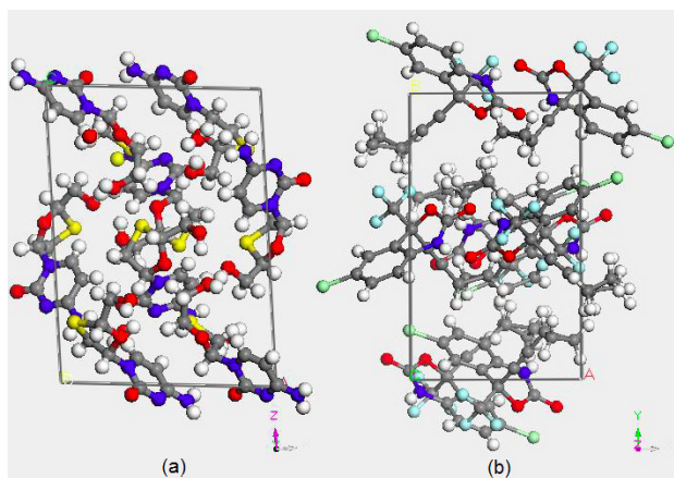
Figure 7. Crystal structure of (a) lamivudine and (b) efavirenz as obtained by Rietveld refinement of the pure samples.
