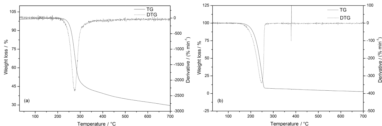
Figure 2. TG and DTG curves of (a) lamivudine and (b) efavirenz.
