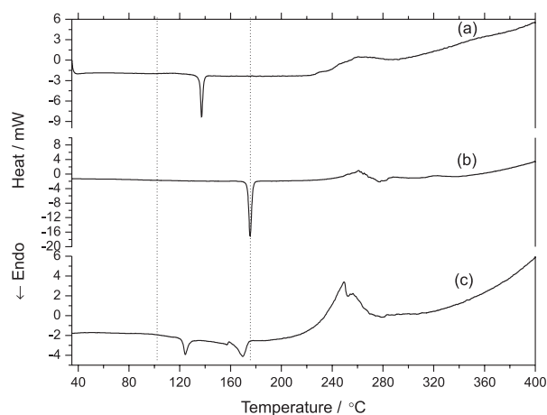
Figure 3. DSC curves of (a) efavirenz, (b) lamivudine and (c) mixture.
