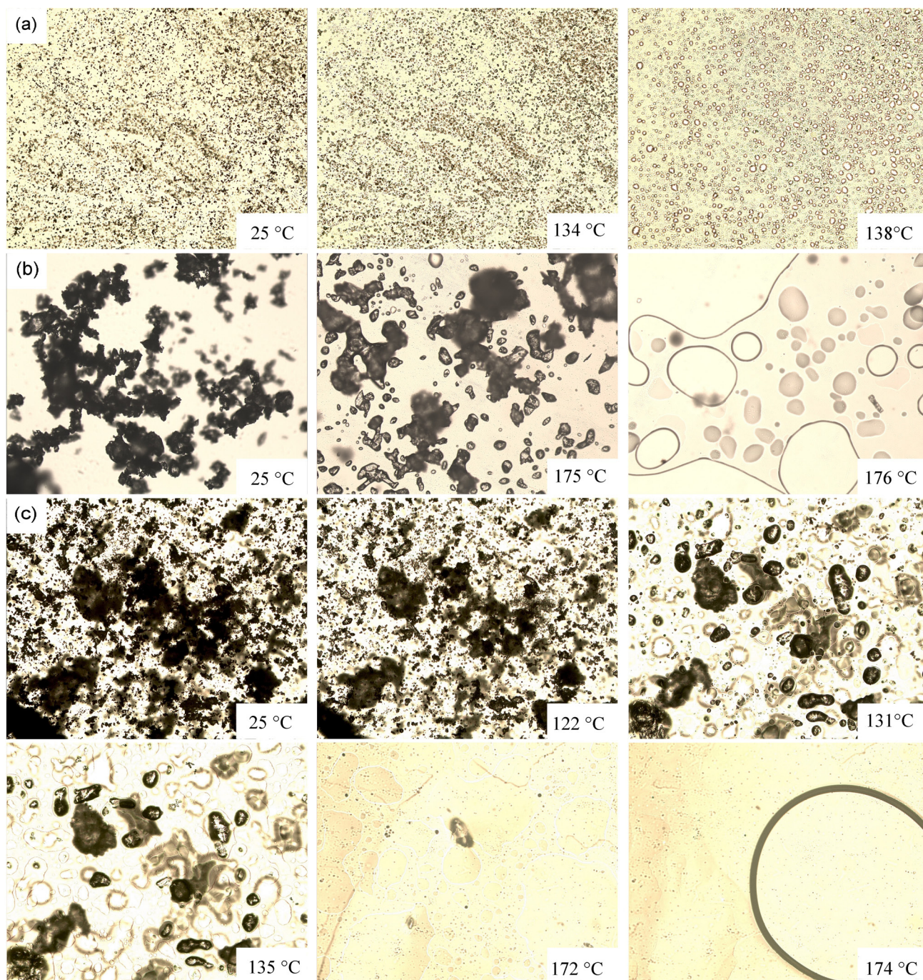
Figure 4. TOA images at 100 \times magnification of (a) efavirenz, (b) lamivudine and (c) mixture. Three images in different temperatures were shown for each pure drug and six for the mixture.
