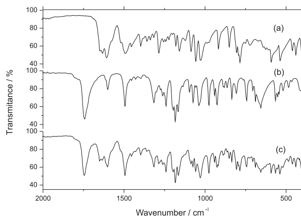
Figure 5. FTIR spectra of (a) lamivudine, (b) efavirenz and (c) mixture.
