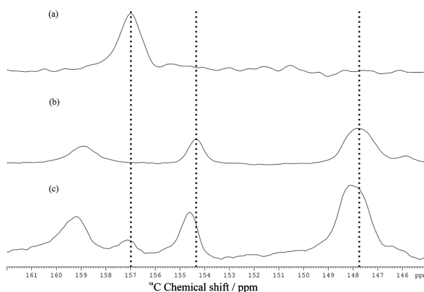
Figure 8. Spectra region amplification of (a) lamivudine, (b) efavirenz and (c) mixture, showing the changes in chemical shifts when drugs are mixed.
