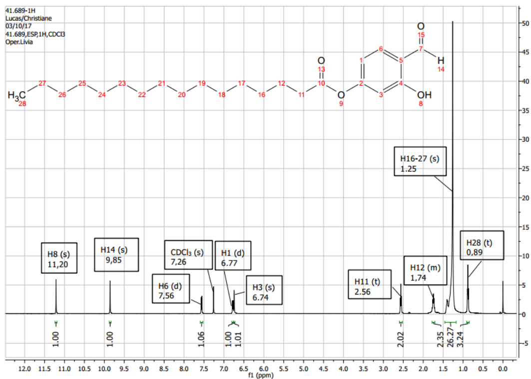
Figure S2. 1 H NMR spectrum (400 MHz, CDCl 3 ) of intermediate ES.
