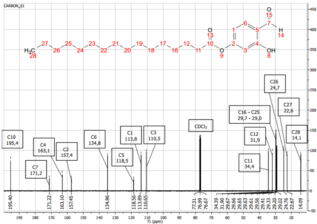
Figure S3. 13 C NMR spectrum (400 MHz, CDCl 3 ) of intermediate ES.
