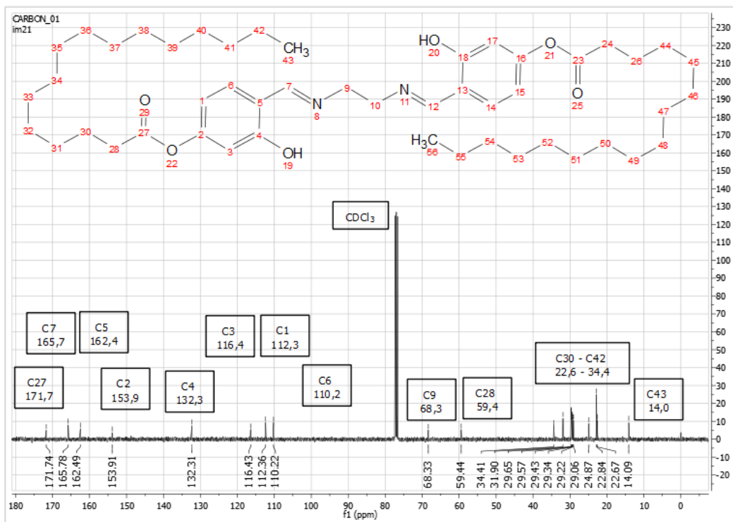
Figure S6. 13 C NMR spectrum (400 MHz, CDCl 3 ) of IM.
