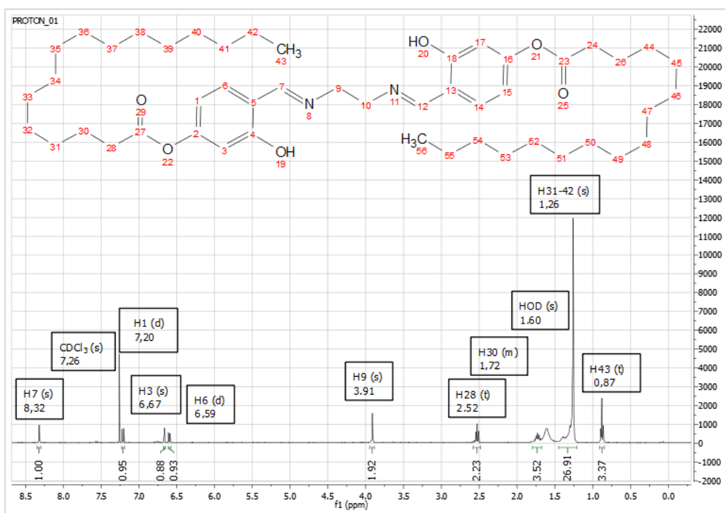
Figure S5. 1 H NMR spectrum (400 MHz, CDCl 3 ) of IM.
