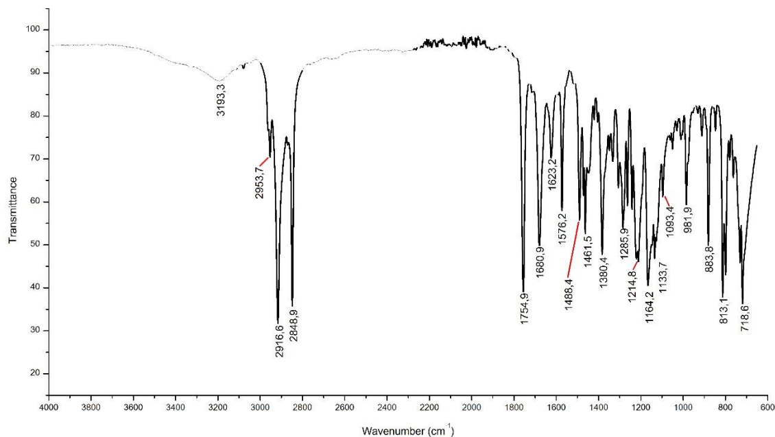
Figure S1. FTIR spectrum of intermediate ES.
