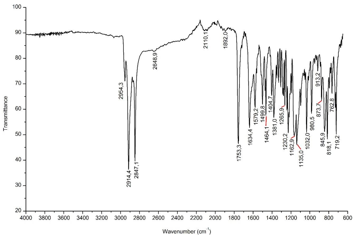
Figure S4. FTIR spectrum of IM.
