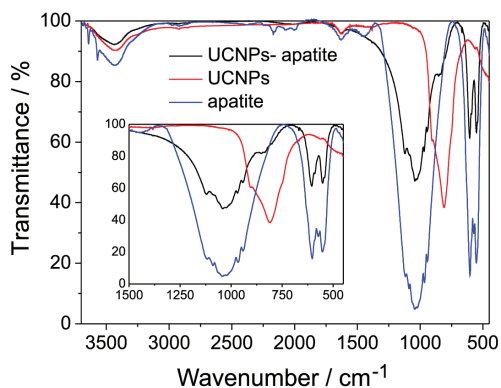
Figure 1. FTIR spectra of UCNPs-apatite, UCNPs and apatite. Inset enlarges the 1500-450 \text{cm}^{-1} region for the exploration.
