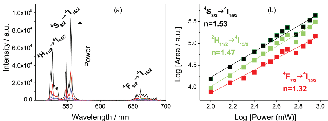
Figure 4. (a) Upconversion emission spectra ( \lambda_{ex} 980 nm) of PCL/UCNPs-apatite scaffold as a function of laser power (100-900 mW). (b) Pump power dependence of the emission intensities.
