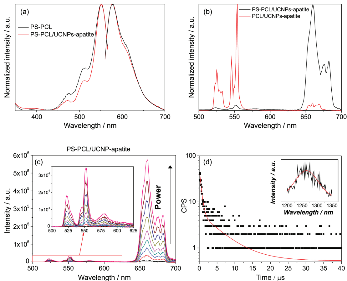
Figure 5. (a) Photoluminescence excitation ( \lambda_{\text{exc}} 575 nm) and emission ( \lambda_{\text{em}} 551 nm) spectra obtained for PS-PCL/UCNPs-apatite and PS-PCL. (b) Up-conversion emission spectra of PCL/UCNPs-apatite and PS-PCL/UCNPs-apatite composites. (c) Up-conversion emission spectra obtained using 980 nm laser pumping at different powers for PS-PCL/UCNPs-apatite composite. The inset shows the amplified spectra in the range from 500 to 625 nm. (d) Singlet oxygen decay curve and exponential fit for PS-PCL/UCNPs-apatite composite in deuterium oxide ( \lambda_{\text{exc}} 980 nm and \lambda_{\text{em}} 1270 nm).
