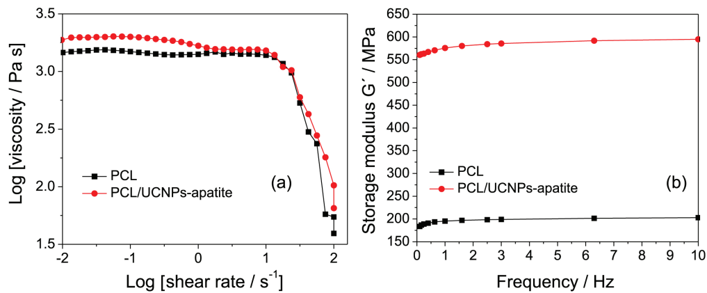
Figure 2. PCL and PCL/UCNPs-apatite. (a) Viscosity as a function of shear rate, at 100 °C and (b) storage modulus as a function of frequency, at 37 °C.
