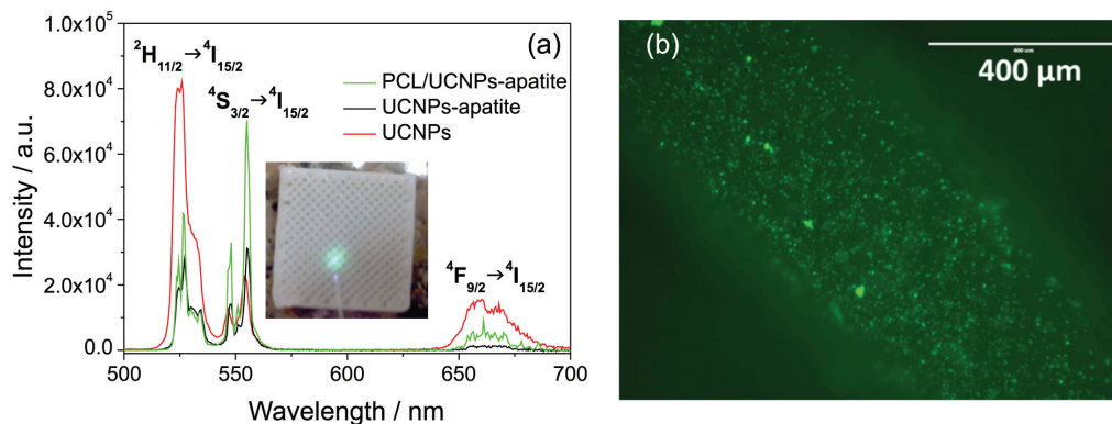
Figure 3. (a) Upconversion emission spectra ( \lambda_{ex} 980 nm) of UCNPs, UCNPs-apatite and PCL/UCNPs-apatite. Inset: corresponding luminescent photograph of the material. (b) Luminescence microscope image of PCL/UCNPs-apatite scaffold.
