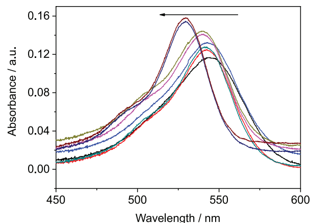
Figure 7. Changes in absorbance intensity of a-Cu II (2.0 μmol L -1 ) measured in DMF-buffer (tris-HCl, 1.0 mmol L -1 , pH 7.4, 1:1, v/v) upon addition of Cys. Cys concentration (from bottom to top): 0, 20, 40, 60, 80, 100, 250, 500 μmol L -1 .
