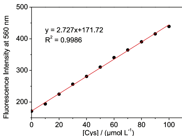
Figure 6. Fluorescent calibration curve of a-Cu II (2.0 μmol L -1 ) as a function of the concentration of Cys (all experiments were performed three times).
