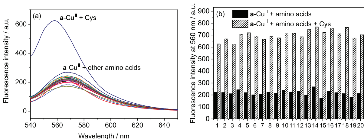
Figure 3. (a) Fluorescence intensity of a-Cu II (2.0 \mu\text{M} ) upon addition of 500 \mu\text{M} of multifarious species in DMF-buffer (tris-HCl, 1.0 \text{mmol L}^{-1} , pH 7.4, 1:1, v/v) (ex: 530 nm; em: 560 nm; slit = 2.5 / 5). (b) Competition graph; 1: blank / Cys, 2: Gly, 3: Glu, 4: Asp, 5: Met, 6: Tyr, 7: Ala, 8: Leu, 9: Ile, 10: Thr, 11: Ser, 12: Pro, 13: Arg, 14: His, 15: Trp, 16: Lys, 17: Val, 18: Phe, 19: Hcy, 20: GSH (reaction time: 20 min).
