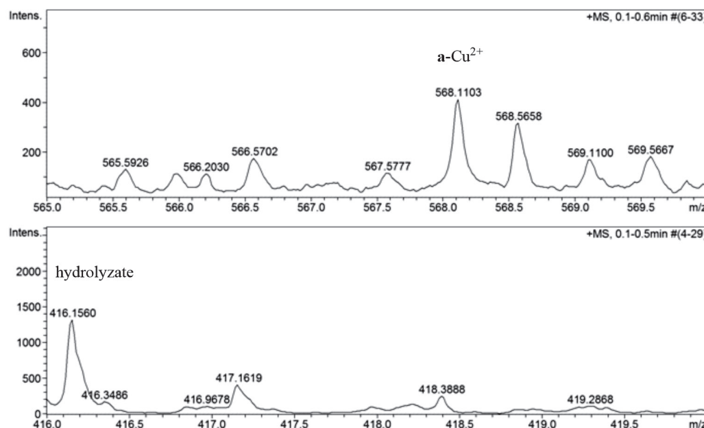
Figure 2. ESI-MS of a - \text{Cu}^{\text{II}} and hydrolyzate.
