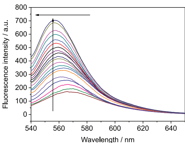
Figure 5. Changes in fluorescent intensity of a-Cu II (2.0 \mu\text{mol L}^{-1} ) measured in DMF-buffer (tris-HCl, 1.0 \text{mmol L}^{-1} , pH 7.4, 1:1, v/v) upon addition of Cys (ex: 530 nm; slit = 2.5 / 5). Cys concentration (from bottom to top): 0, 10, 20, 30, 40, 50, 60, 70, 80, 90, 100, 150, 180, 200, 250, 300, 350, 400, 450, 500 \mu\text{mol L}^{-1} .
