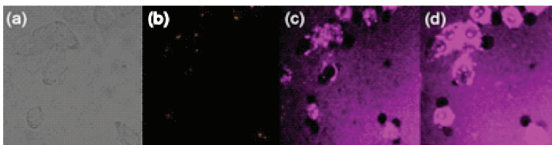
Figure 8. Confocal fluorescence images of sensor (Olympus FV1000). (a) Bright-field transmission image; (b) fluorescence image of cells incubated with 20 μmol L -1 of a-Cu II and NEM (1000 μmol L -1 ) (λ ex = 488 nm); (c) fluorescence image of cells incubated with 20 μmol L -1 of a-Cu II and NEM (500 μmol L -1 ) (λ ex = 488 nm); (d) fluorescence image of cells incubated with 20 μmol L -1 of a-Cu II (λ ex = 488 nm).
