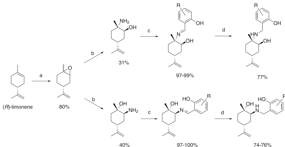
Scheme 1. Present work overview.
