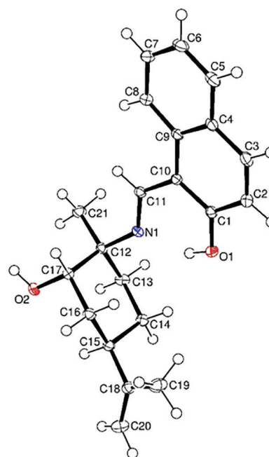
Figure 2. Molecular structure of 6a with the key atoms labelled (thermal ellipsoids drawn at 50% probability level).
