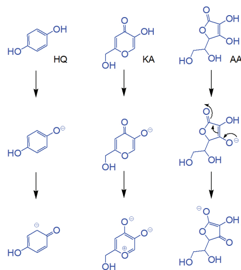
Scheme 2. Resonance structures of the hydroquinone and related derivatives.
