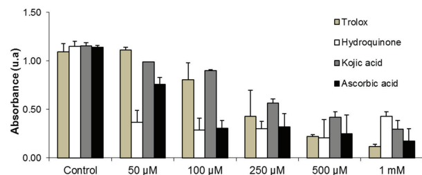
Figure 3. Antioxidant evaluation of the hydroquinone, kojic acid, ascorbic acid, and trolox using DPPH radical.
