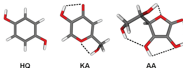
Figure 4. Structure of the hydroquinone and related derivatives.
