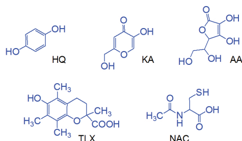
Scheme 1. Chemical structures of the hydroquinone, related derivatives, and antioxidants.
