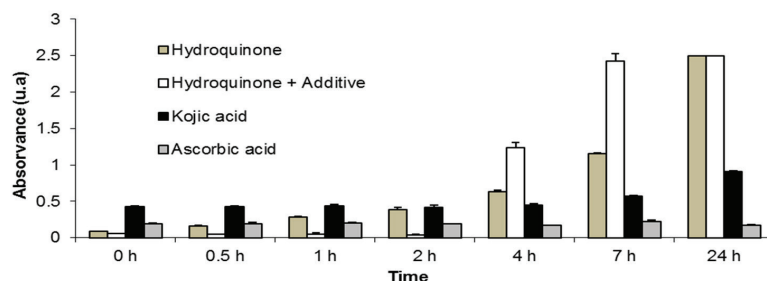
Figure 1. Chemistry stability for the hydroquinone, hydroquinone + additive (NAC), kojic acid, and ascorbic acid in alkaline solution (water:ethanol 1:1, sodium bicarbonate 0.05%). p < 0.01 vs. control (0 h), (ANOVA, Tukey's range test).
