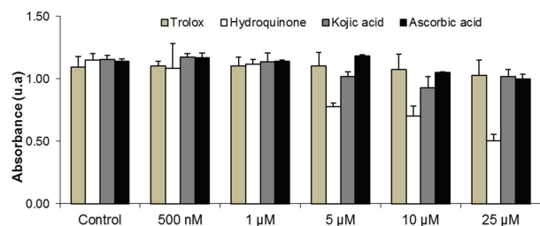
Figure 2. Antioxidant evaluation of the hydroquinone, kojic acid, ascorbic acid, and trolox using DPPH radical.
