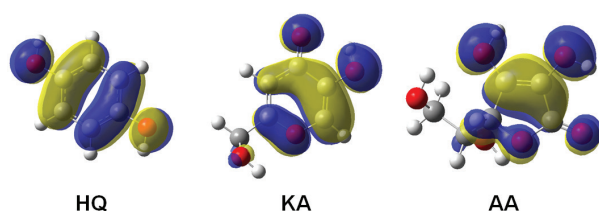
Figure 5. HOMO of the hydroquinone and related derivatives.
