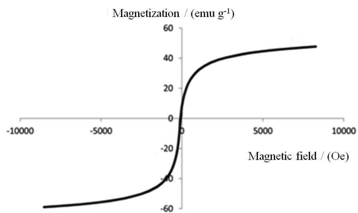
Figure S3. Magnetization curve of Fe 3 O 4 nanoparticles.
