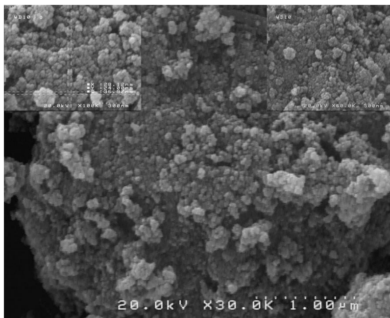
Figure S2. FE-SEM images of Fe 3 O 4 .
