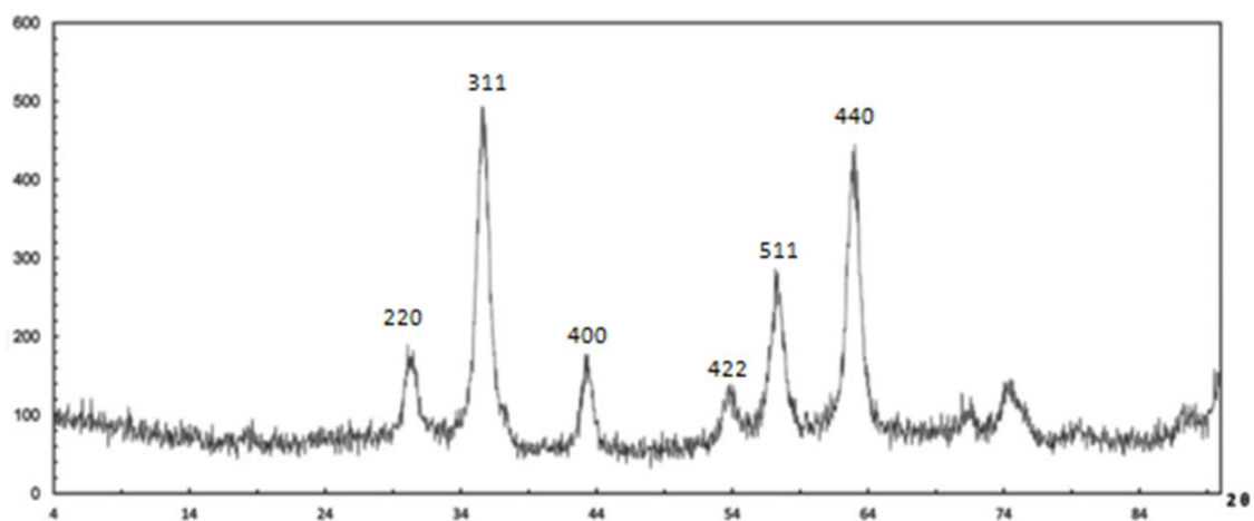
Figure S1. X-Ray diffraction pattern of Fe 3 O 4 .
