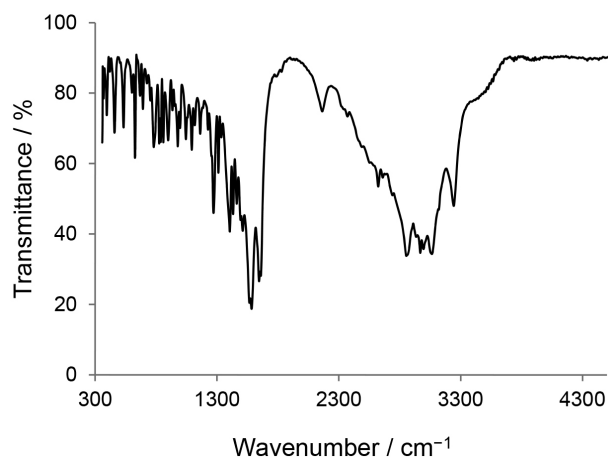
Figure S1. FTIR (KBr) spectrum of compound 7.
