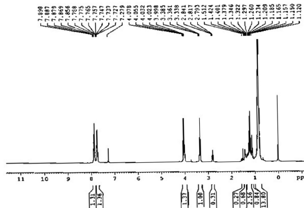
Figure S2. 1 H NMR spectrum (300 MHz, D 2 O) of compound 7.
