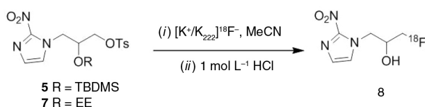
Scheme 2. Radiosynthesis of [ ^{18}\text{F} ]FMISO from new FMISO precursors.
