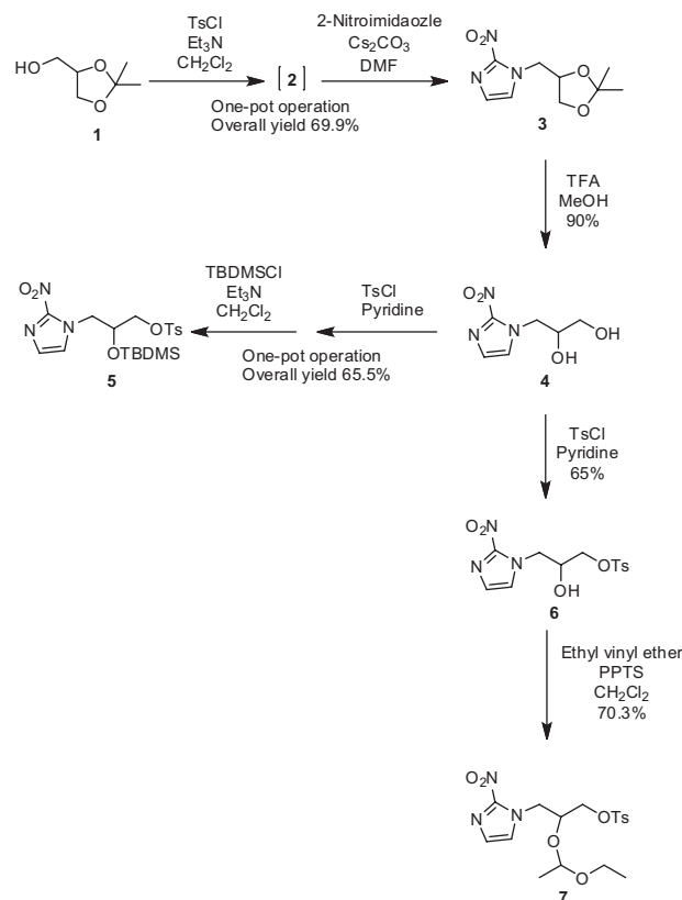
Scheme 1. Synthesis of [ ^{18}\text{F} ]FMISO precursors from 2,2-dimethyl-1,3-dioxolane-4-methanol.
