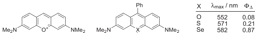
Figure 14. Pyronin and simple rosamine derivatives.
