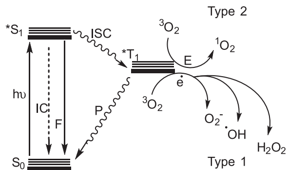
Figure 1. Excitation/relaxation pathways involved in photosensitisation. Key: S_0 : singlet electronic ground state of photosensitiser; *S_1 : singlet excited state; *T_1 : triplet excited state; h\nu : energy of absorbed photon; IC: internal conversion; F: fluorescence; P: phosphorescence; ISC: inter-system crossing.
