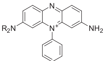
R = H, Phenosafranin R = Et, Methylene violet 3RAX
