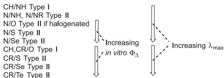
Figure 18. Structure-photophysical relationships in cationic, azine-type photosensitisers.
