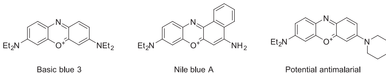
Figure 8. Phenoxazinium derivatives.
