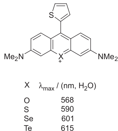
Figure 17. Effect of lower period atom inclusion in rosamine derivatives.
