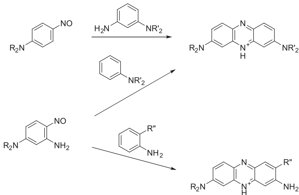
Figure 6. Classical synthesis of phenazinium dyes showing facile variation. Typically R is an alkyl group.
